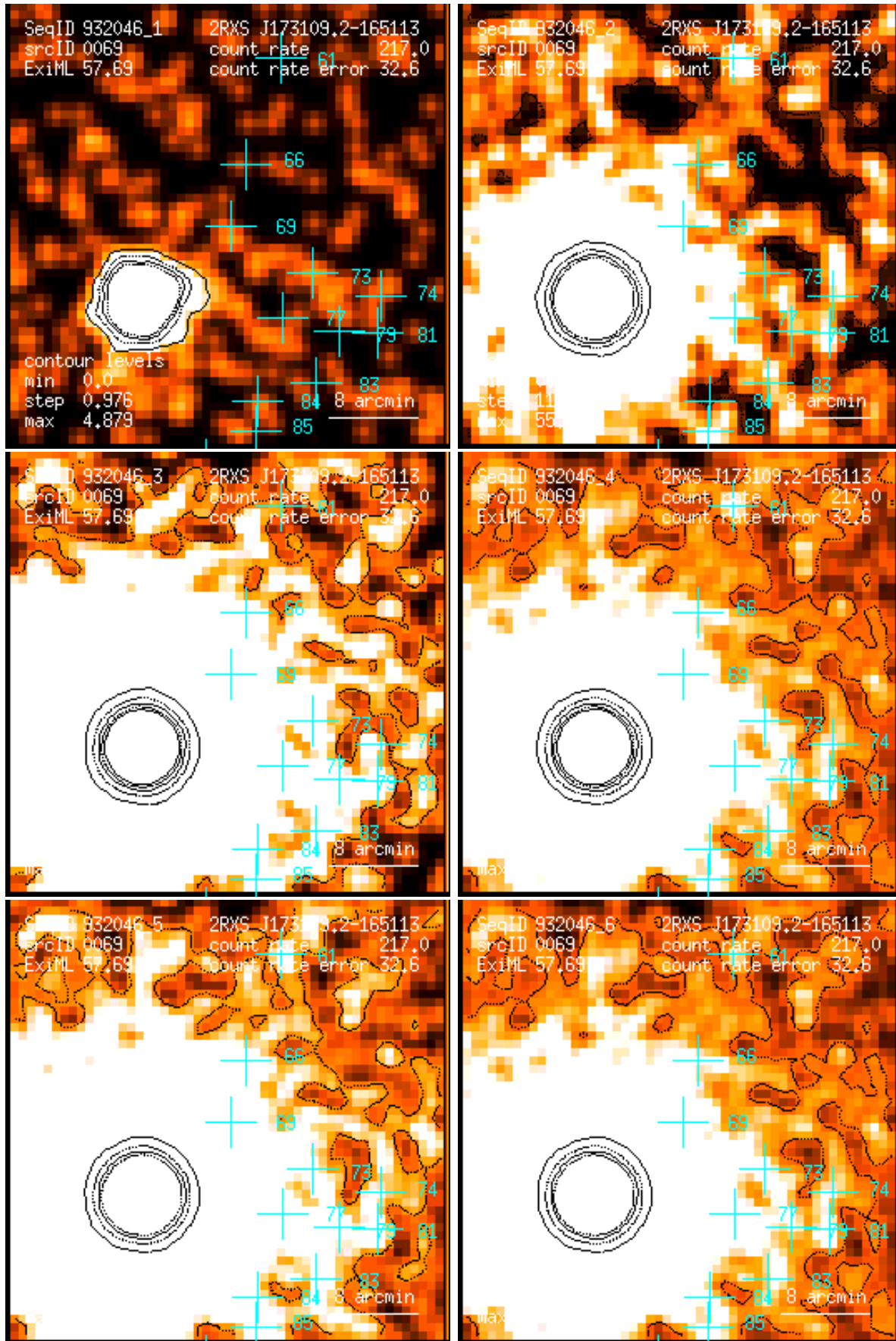
Figure 69: RASS 932046: detection 0069: band rate images, Gaussian filter: (1) PSPC channels 11 – 41, (2) 52 – 90, (3) 91 – 201, (4) 11 – 235, (5) 52 – 201, (6) 11 – 201. Broad band rates in counts/ks. Band rate contour levels in counts/ks/arcmin 2 .
