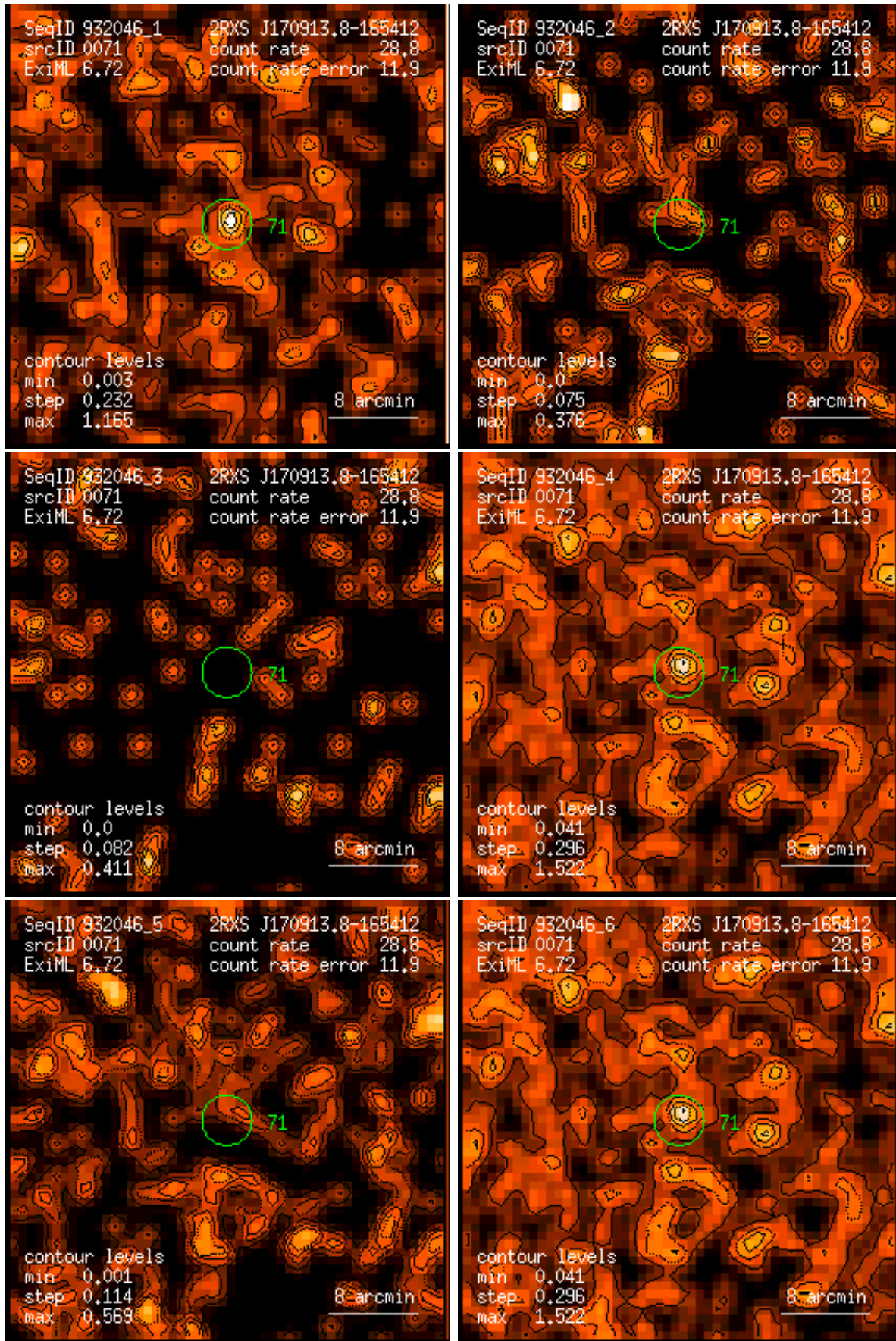
Figure 71: RASS 932046: detection 0071: band rate images, Gaussian filter: (1) PSPC channels 11 – 41, (2) 52 – 90, (3) 91 – 201, (4) 11 – 235, (5) 52 – 201, (6) 11 – 201. Broad band rates in counts/ks. Band rate contour levels in counts/ks/arcmin 2 .
