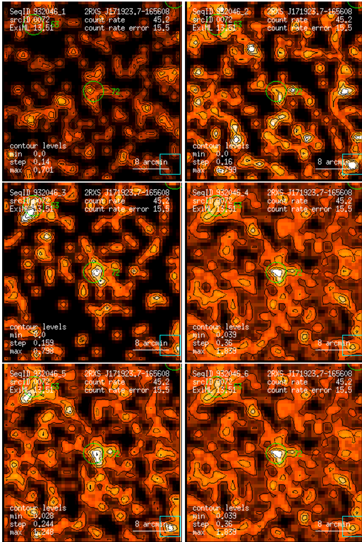
Figure 72: RASS 932046: detection 0072: band rate images, Gaussian filter: (1) PSPC channels 11 – 41, (2) 52 – 90, (3) 91 – 201, (4) 11 – 235, (5) 52 – 201, (6) 11 – 201. Broad band rates in counts/ks. Band rate contour levels in counts/ks/arcmin 2 .
