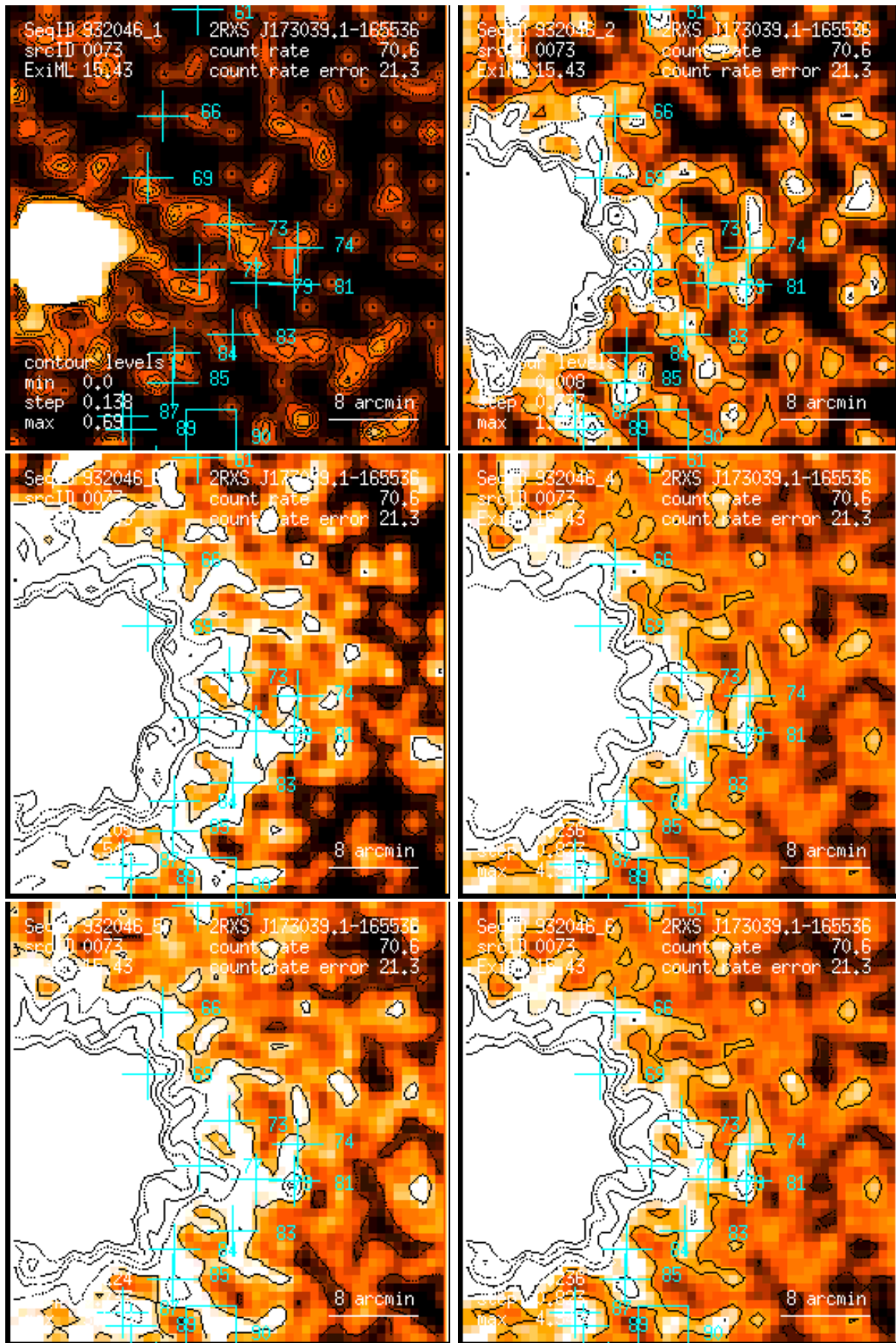
Figure 73: RASS 932046: detection 0073: band rate images, Gaussian filter: (1) PSPC channels 11 – 41, (2) 52 – 90, (3) 91 – 201, (4) 11 – 235, (5) 52 – 201, (6) 11 – 201. Broad band rates in counts/ks. Band rate contour levels in counts/ks/arcmin 2 .
