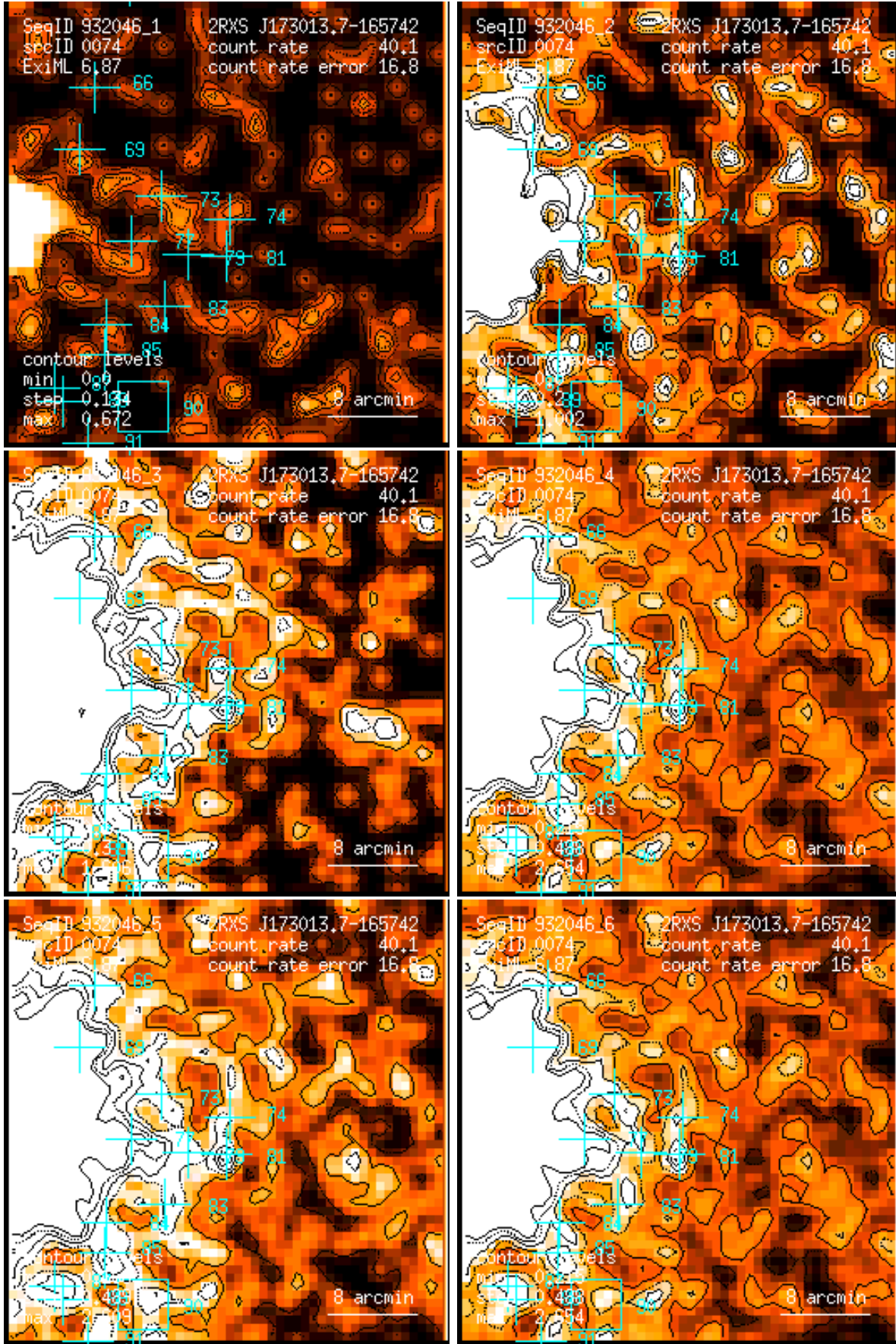
Figure 74: RASS 932046: detection 0074: band rate images, Gaussian filter: (1) PSPC channels 11 – 41, (2) 52 – 90, (3) 91 – 201, (4) 11 – 235, (5) 52 – 201, (6) 11 – 201. Broad band rates in counts/ks. Band rate contour levels in counts/ks/arcmin 2 .
