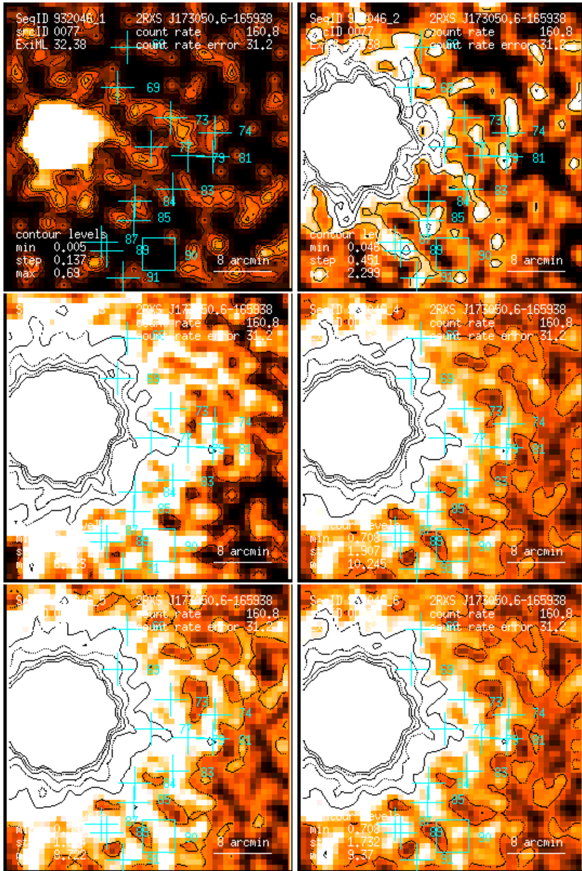
Figure 77: RASS 932046: detection 0077: band rate images, Gaussian filter: (1) PSPC channels 11 – 41, (2) 52 – 90, (3) 91 – 201, (4) 11 – 235, (5) 52 – 201, (6) 11 – 201. Broad band rates in counts/ks. Band rate contour levels in counts/ks/arcmin 2 .
