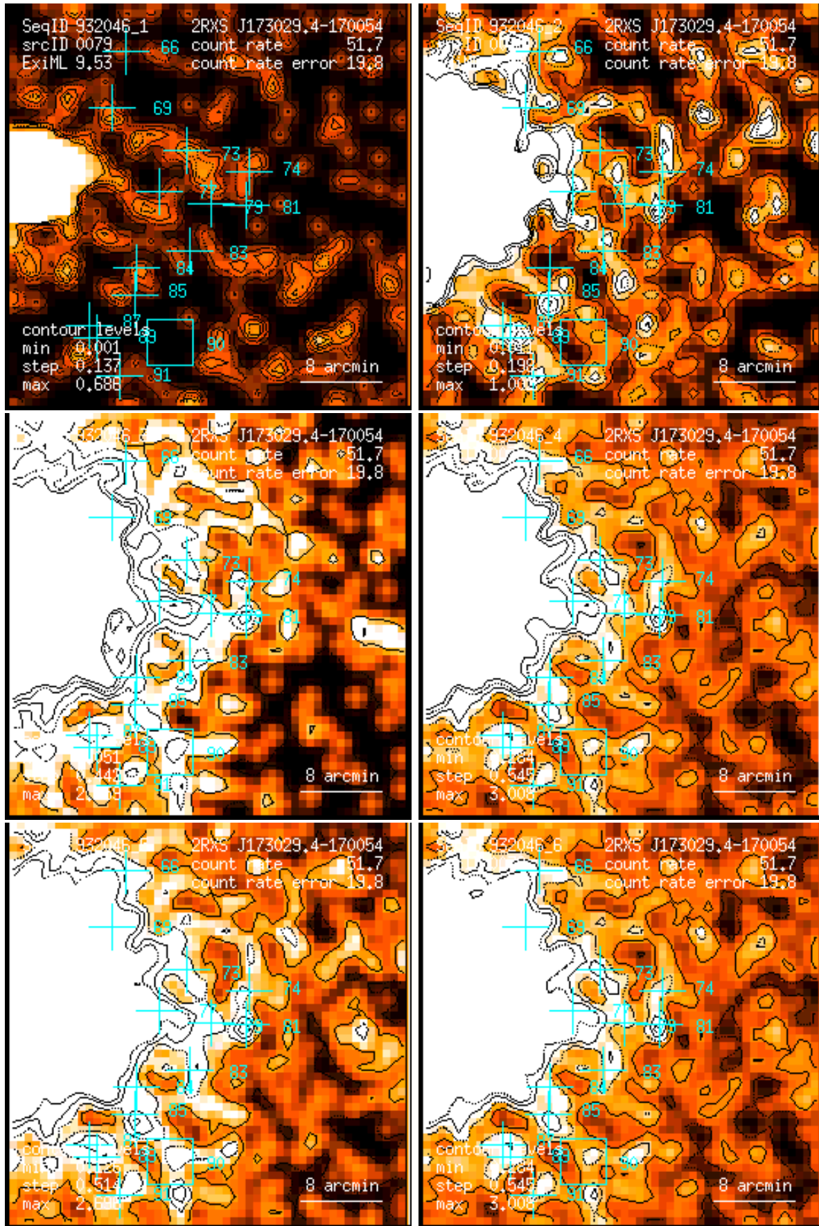
Figure 79: RASS 932046: detection 0079: band rate images, Gaussian filter: (1) PSPC channels 11 – 41, (2) 52 – 90, (3) 91 – 201, (4) 11 – 235, (5) 52 – 201, (6) 11 – 201. Broad band rates in counts/ks. Band rate contour levels in counts/ks/arcmin 2 .
