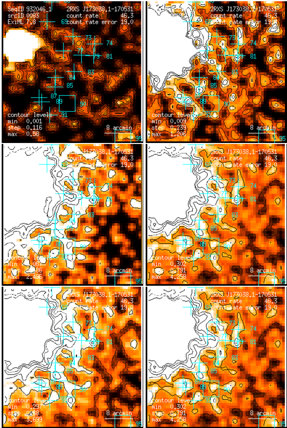
Figure 83: RASS 932046: detection 0083: band rate images, Gaussian filter: (1) PSPC channels 11 – 41, (2) 52 – 90, (3) 91 – 201, (4) 11 – 235, (5) 52 – 201, (6) 11 – 201. Broad band rates in counts/ks. Band rate contour levels in counts/ks/arcmin 2 .
