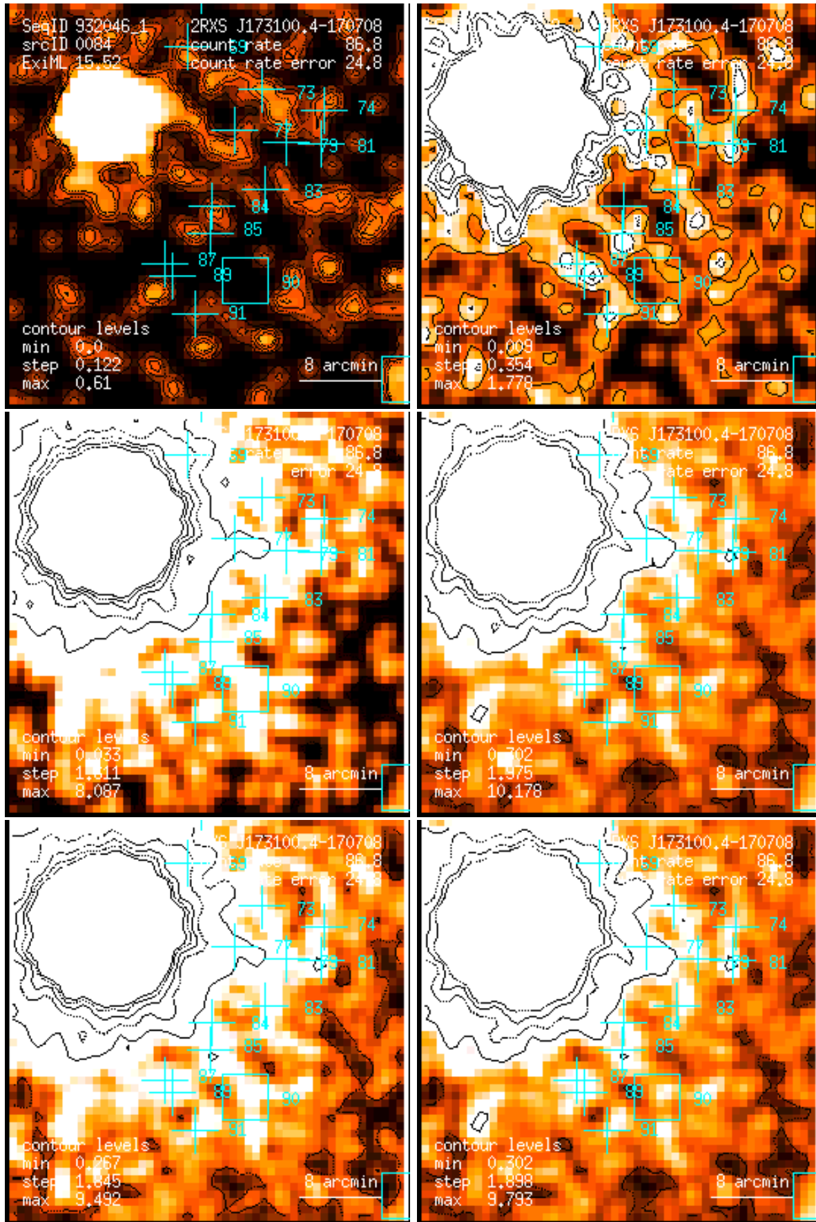
Figure 84: RASS 932046: detection 0084: band rate images, Gaussian filter: (1) PSPC channels 11 – 41, (2) 52 – 90, (3) 91 – 201, (4) 11 – 235, (5) 52 – 201, (6) 11 – 201. Broad band rates in counts/ks. Band rate contour levels in counts/ks/arcmin 2 .
