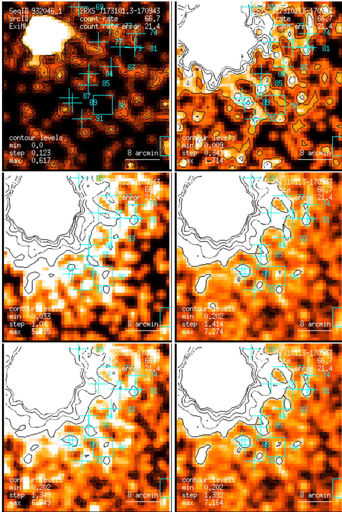
Figure 85: RASS 932046: detection 0085: band rate images, Gaussian filter: (1) PSPC channels 11 – 41, (2) 52 – 90, (3) 91 – 201, (4) 11 – 235, (5) 52 – 201, (6) 11 – 201. Broad band rates in counts/ks. Band rate contour levels in counts/ks/arcmin 2 .
