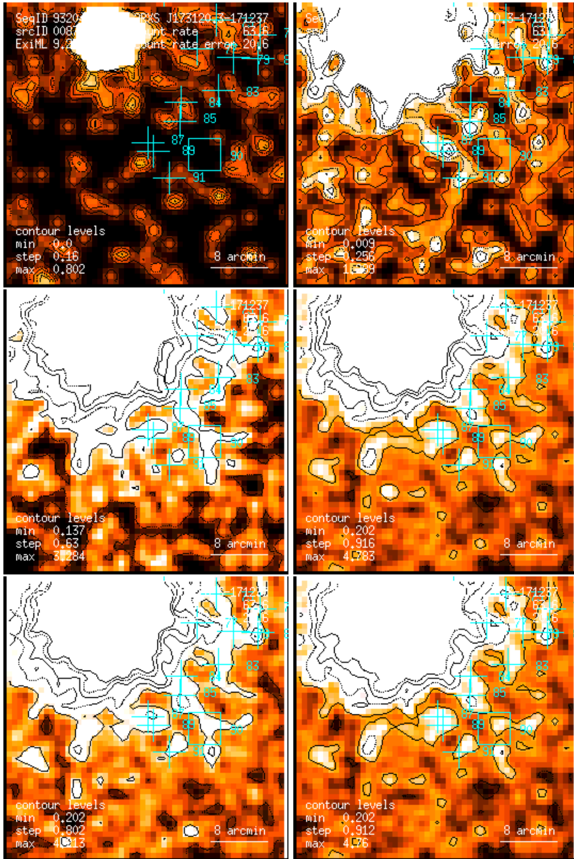
Figure 87: RASS 932046: detection 0087: band rate images, Gaussian filter: (1) PSPC channels 11 – 41, (2) 52 – 90, (3) 91 – 201, (4) 11 – 235, (5) 52 – 201, (6) 11 – 201. Broad band rates in counts/ks. Band rate contour levels in counts/ks/arcmin 2 .
