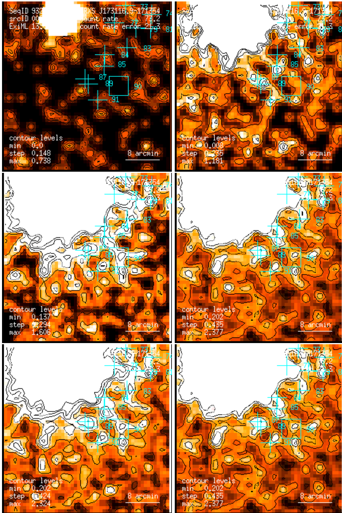
Figure 89: RASS 932046: detection 0089: band rate images, Gaussian filter: (1) PSPC channels 11 – 41, (2) 52 – 90, (3) 91 – 201, (4) 11 – 235, (5) 52 – 201, (6) 11 – 201. Broad band rates in counts/ks. Band rate contour levels in counts/ks/arcmin 2 .
