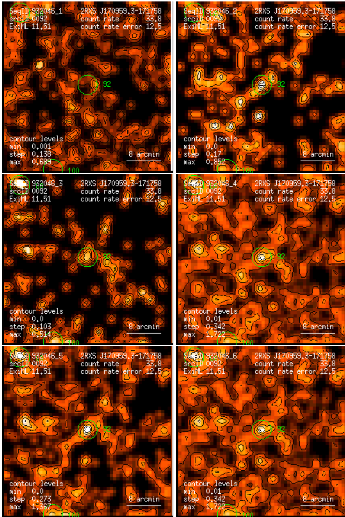
Figure 92: RASS 932046: detection 0092: band rate images, Gaussian filter: (1) PSPC channels 11 – 41, (2) 52 – 90, (3) 91 – 201, (4) 11 – 235, (5) 52 – 201, (6) 11 – 201. Broad band rates in counts/ks. Band rate contour levels in counts/ks/arcmin 2 .
