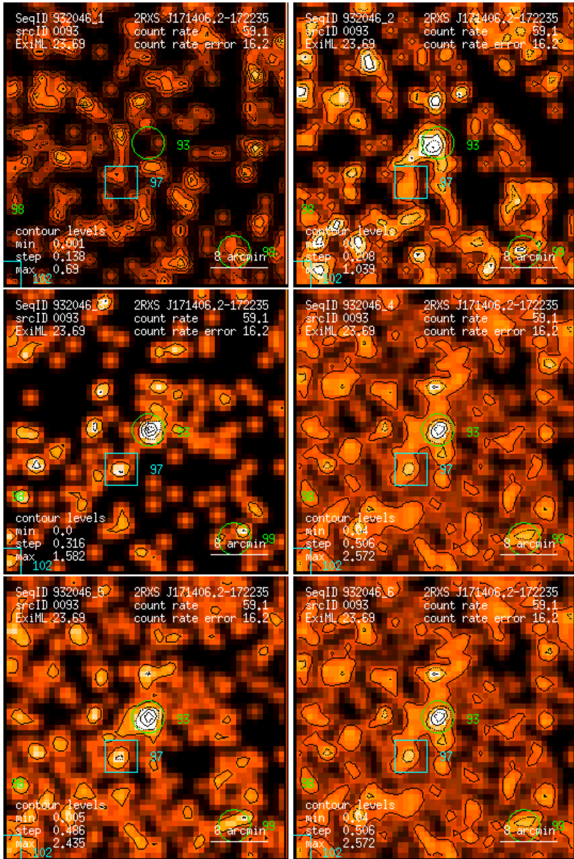
Figure 93: RASS 932046: detection 0093: band rate images, Gaussian filter: (1) PSPC channels 11 – 41, (2) 52 – 90, (3) 91 – 201, (4) 11 – 235, (5) 52 – 201, (6) 11 – 201. Broad band rates in counts/ks. Band rate contour levels in counts/ks/arcmin 2 .
