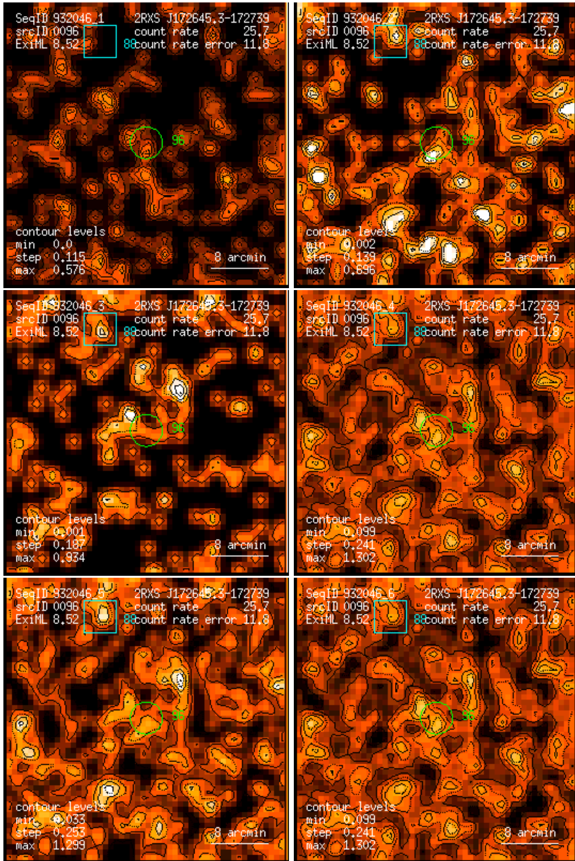
Figure 96: RASS 932046: detection 0096: band rate images, Gaussian filter: (1) PSPC channels 11 – 41, (2) 52 – 90, (3) 91 – 201, (4) 11 – 235, (5) 52 – 201, (6) 11 – 201. Broad band rates in counts/ks. Band rate contour levels in counts/ks/arcmin 2 .
