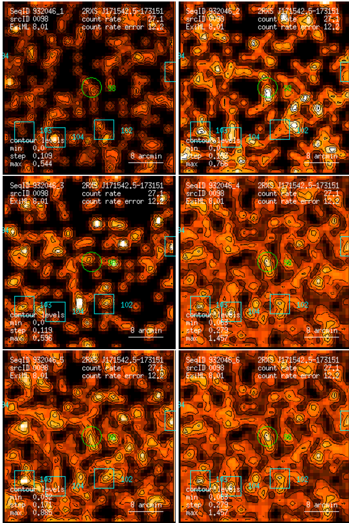
Figure 98: RASS 932046: detection 0098: band rate images, Gaussian filter: (1) PSPC channels 11 – 41, (2) 52 – 90, (3) 91 – 201, (4) 11 – 235, (5) 52 – 201, (6) 11 – 201. Broad band rates in counts/ks. Band rate contour levels in counts/ks/arcmin 2 .
