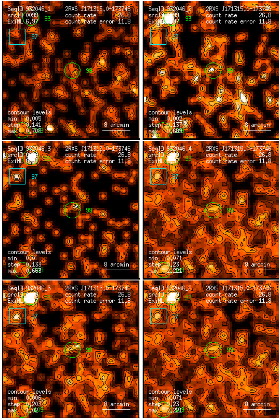
Figure 99: RASS 932046: detection 0099: band rate images, Gaussian filter: (1) PSPC channels 11 – 41, (2) 52 – 90, (3) 91 – 201, (4) 11 – 235, (5) 52 – 201, (6) 11 – 201. Broad band rates in counts/ks. Band rate contour levels in counts/ks/arcmin 2 .
