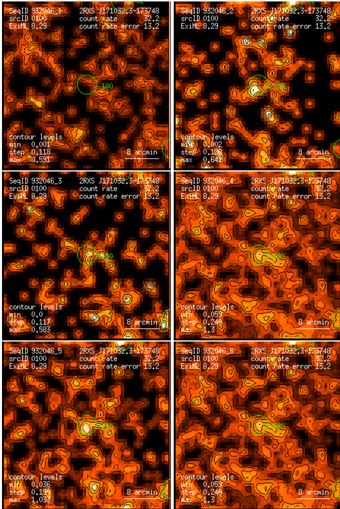
Figure 100: RASS 932046: detection 0100: band rate images, Gaussian filter: (1) PSPC channels 11 – 41, (2) 52 – 90, (3) 91 – 201, (4) 11 – 235, (5) 52 – 201, (6) 11 – 201. Broad band rates in counts/ks. Band rate contour levels in counts/ks/arcmin 2 .
