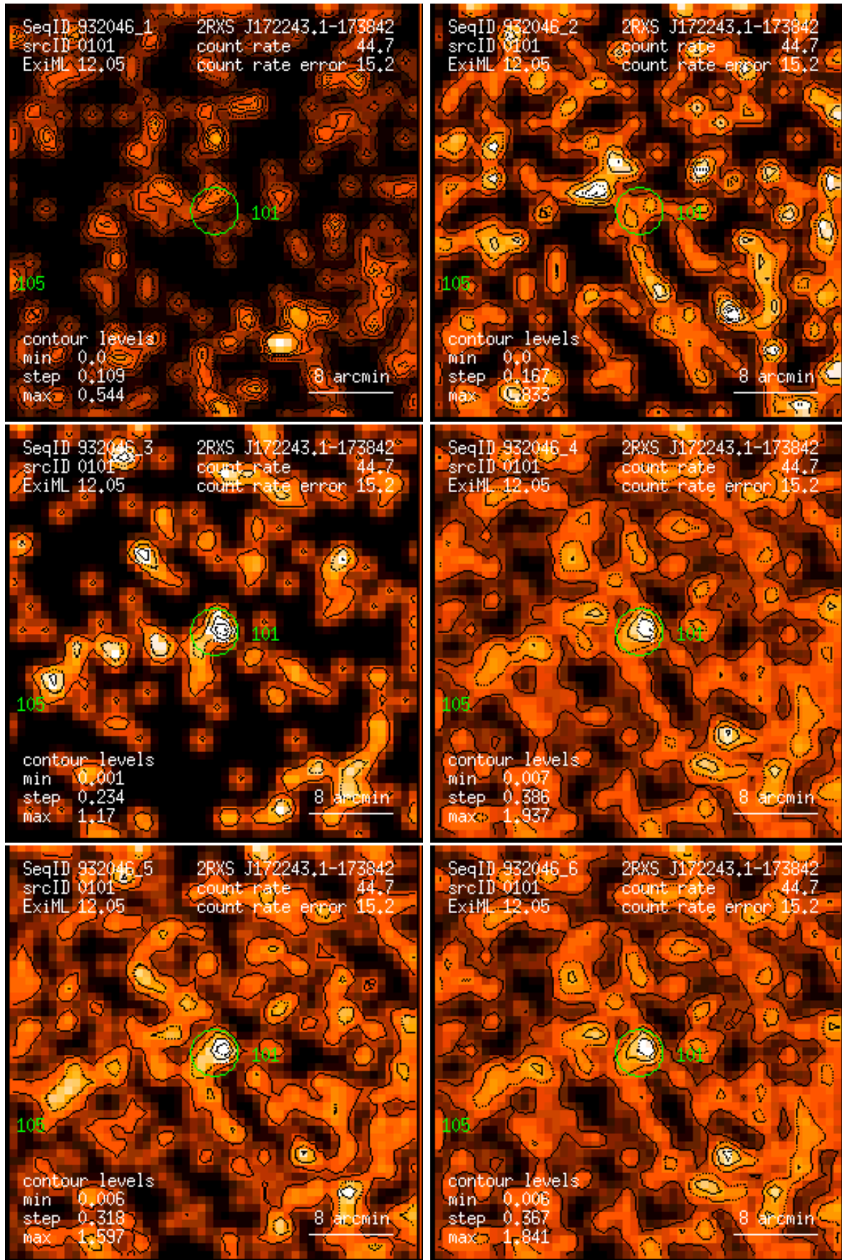
Figure 101: RASS 932046: detection 0101: band rate images, Gaussian filter: (1) PSPC channels 11 – 41, (2) 52 – 90, (3) 91 – 201, (4) 11 – 235, (5) 52 – 201, (6) 11 – 201. Broad band rates in counts/ks. Band rate contour levels in counts/ks/arcmin 2 .
