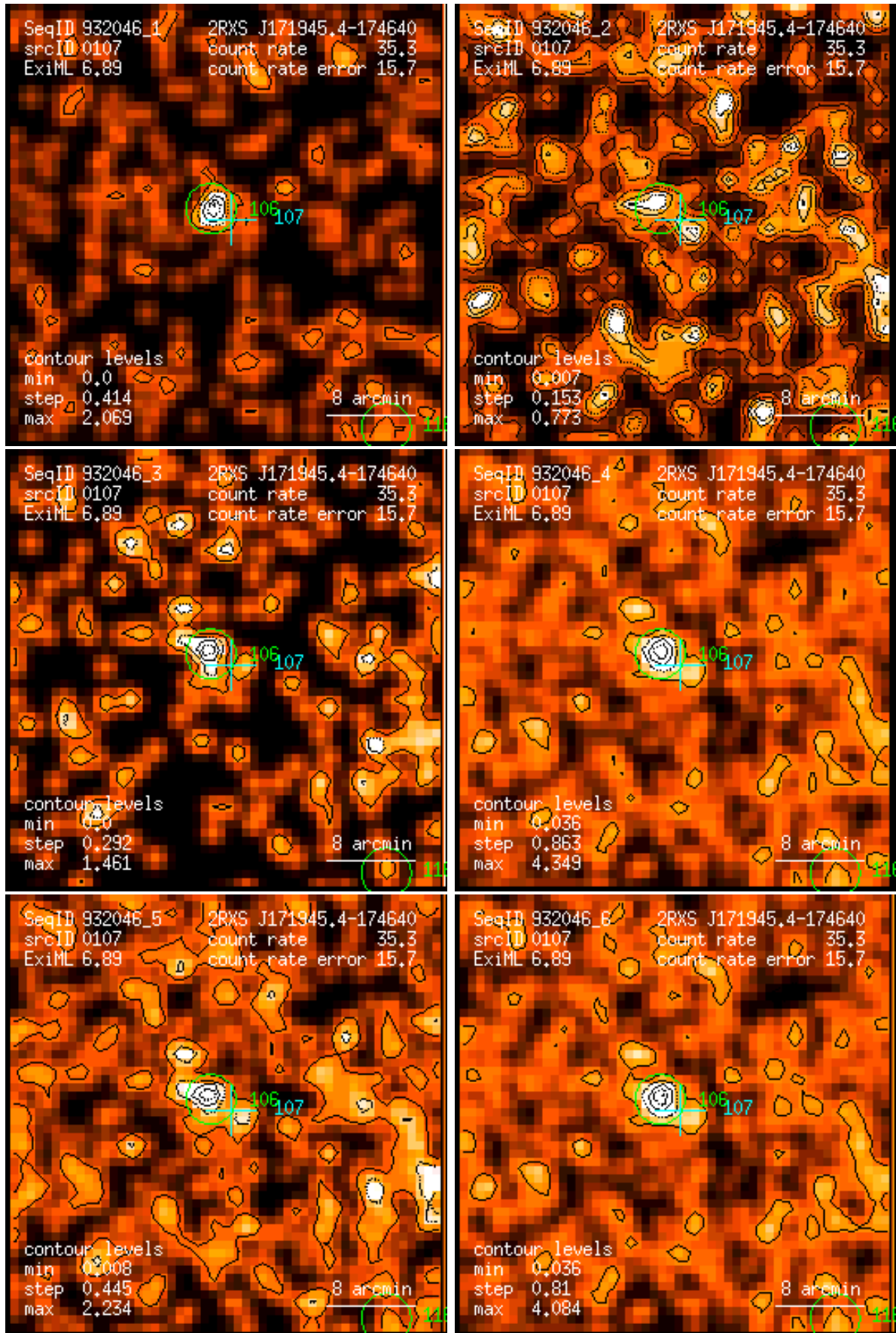
Figure 107: RASS 932046: detection 0107: band rate images, Gaussian filter: (1) PSPC channels 11 – 41, (2) 52 – 90, (3) 91 – 201, (4) 11 – 235, (5) 52 – 201, (6) 11 – 201. Broad band rates in counts/ks. Band rate contour levels in counts/ks/arcmin 2 .
