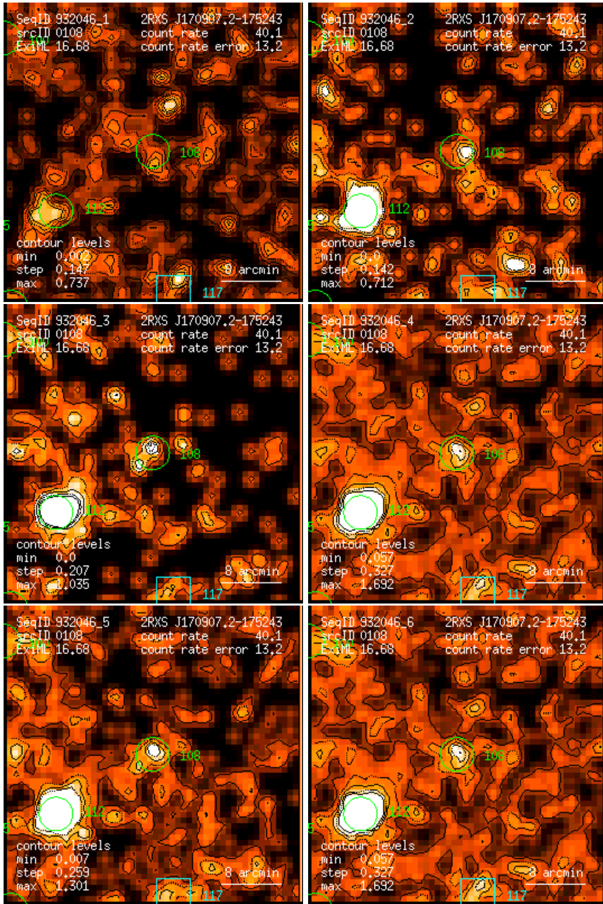
Figure 108: RASS 932046: detection 0108: band rate images, Gaussian filter: (1) PSPC channels 11 – 41, (2) 52 – 90, (3) 91 – 201, (4) 11 – 235, (5) 52 – 201, (6) 11 – 201. Broad band rates in counts/ks. Band rate contour levels in counts/ks/arcmin 2 .
