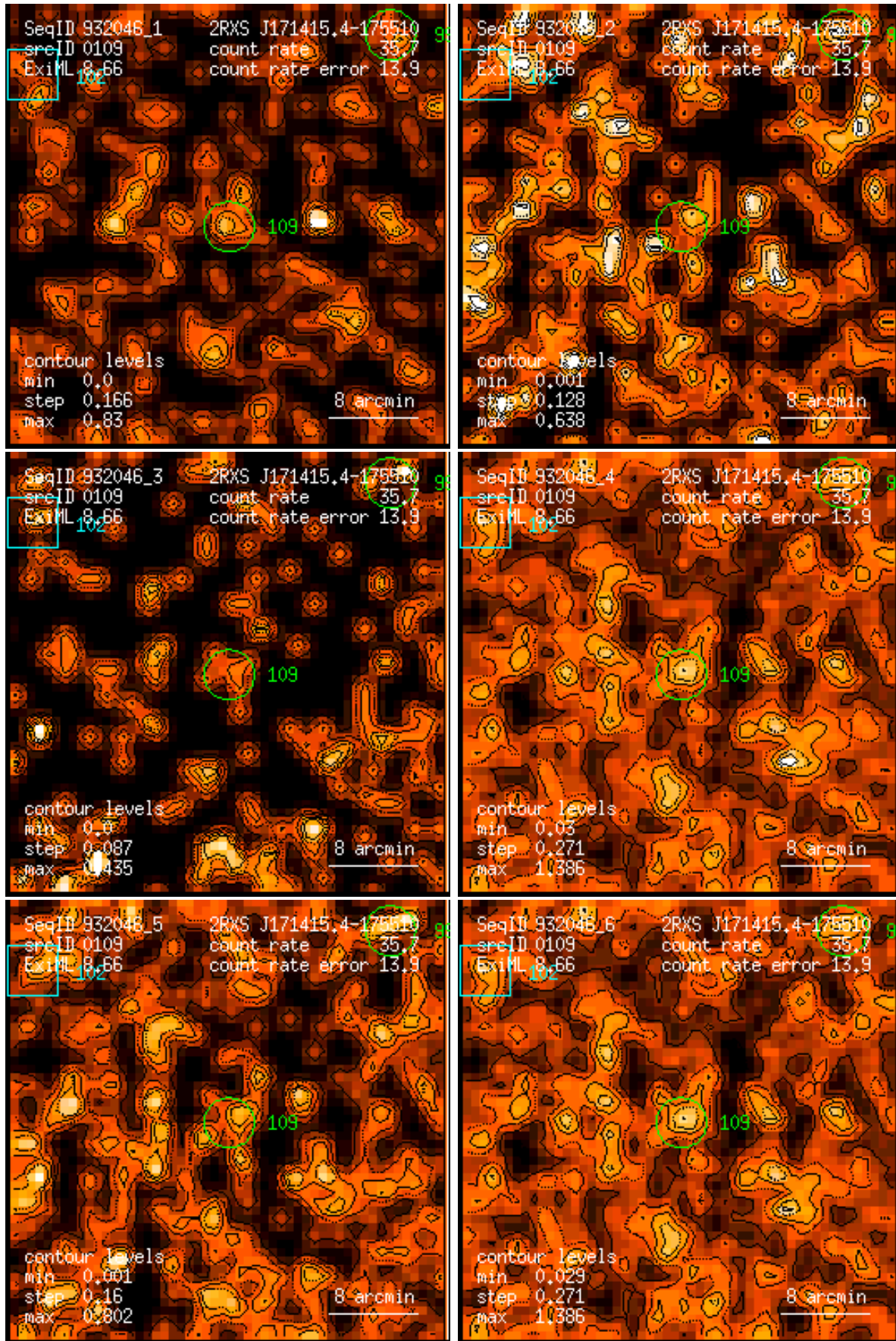
Figure 109: RASS 932046: detection 0109: band rate images, Gaussian filter: (1) PSPC channels 11 – 41, (2) 52 – 90, (3) 91 – 201, (4) 11 – 235, (5) 52 – 201, (6) 11 – 201. Broad band rates in counts/ks. Band rate contour levels in counts/ks/arcmin 2 .
