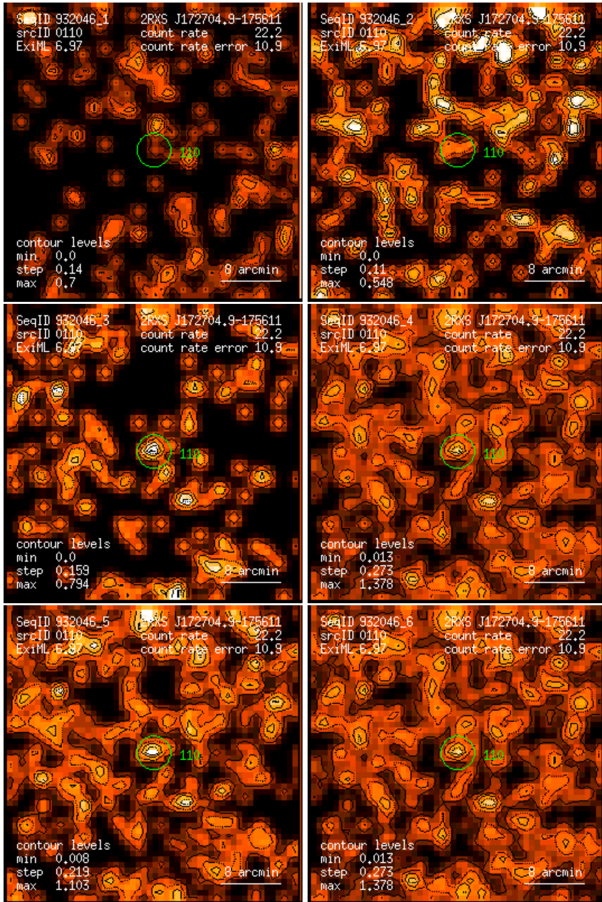
Figure 110: RASS 932046: detection 0110: band rate images, Gaussian filter: (1) PSPC channels 11 – 41, (2) 52 – 90, (3) 91 – 201, (4) 11 – 235, (5) 52 – 201, (6) 11 – 201. Broad band rates in counts/ks. Band rate contour levels in counts/ks/arcmin 2 .
