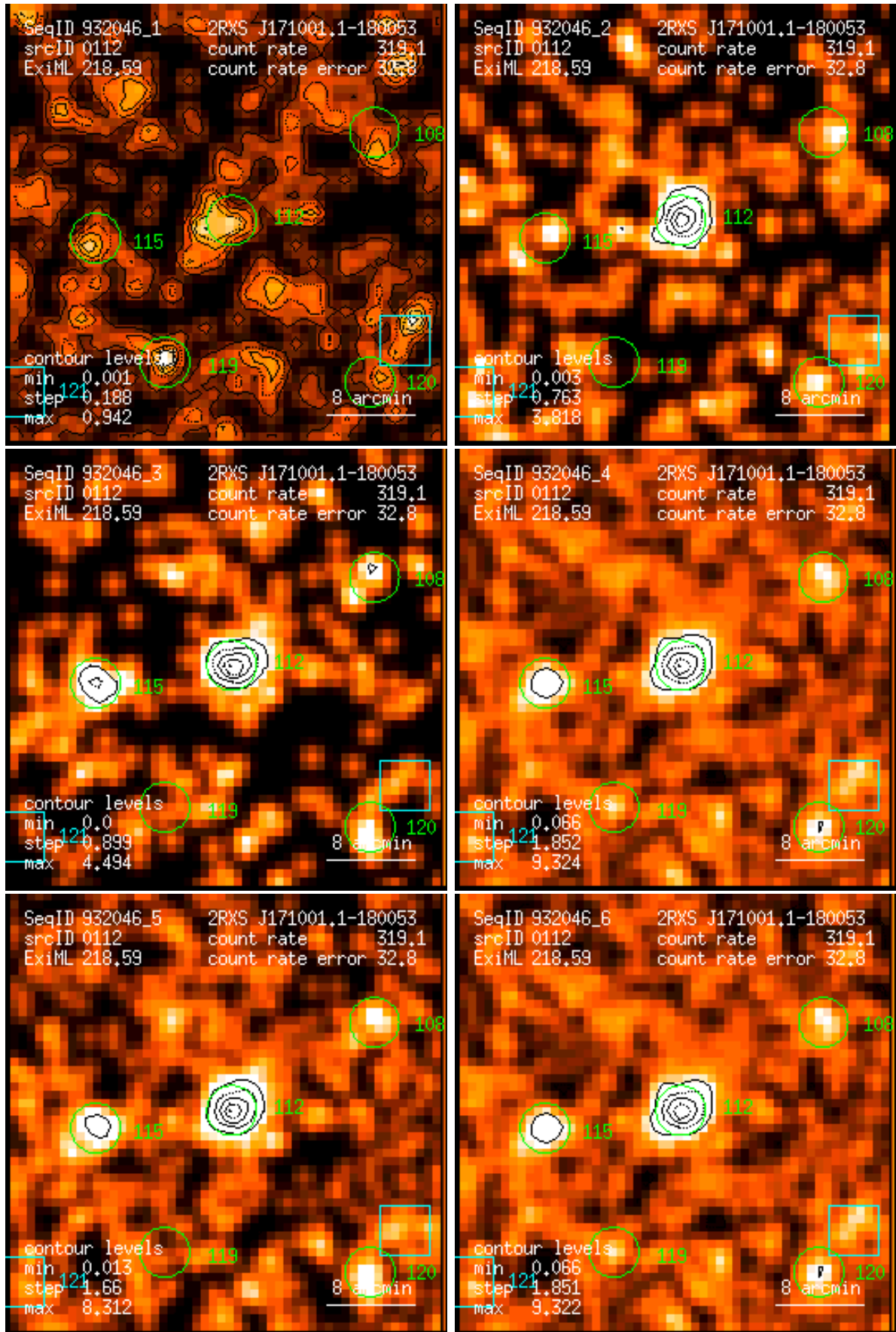
Figure 112: RASS 932046: detection 0112: band rate images, Gaussian filter: (1) PSPC channels 11 – 41, (2) 52 – 90, (3) 91 – 201, (4) 11 – 235, (5) 52 – 201, (6) 11 – 201. Broad band rates in counts/ks. Band rate contour levels in counts/ks/arcmin 2 .
