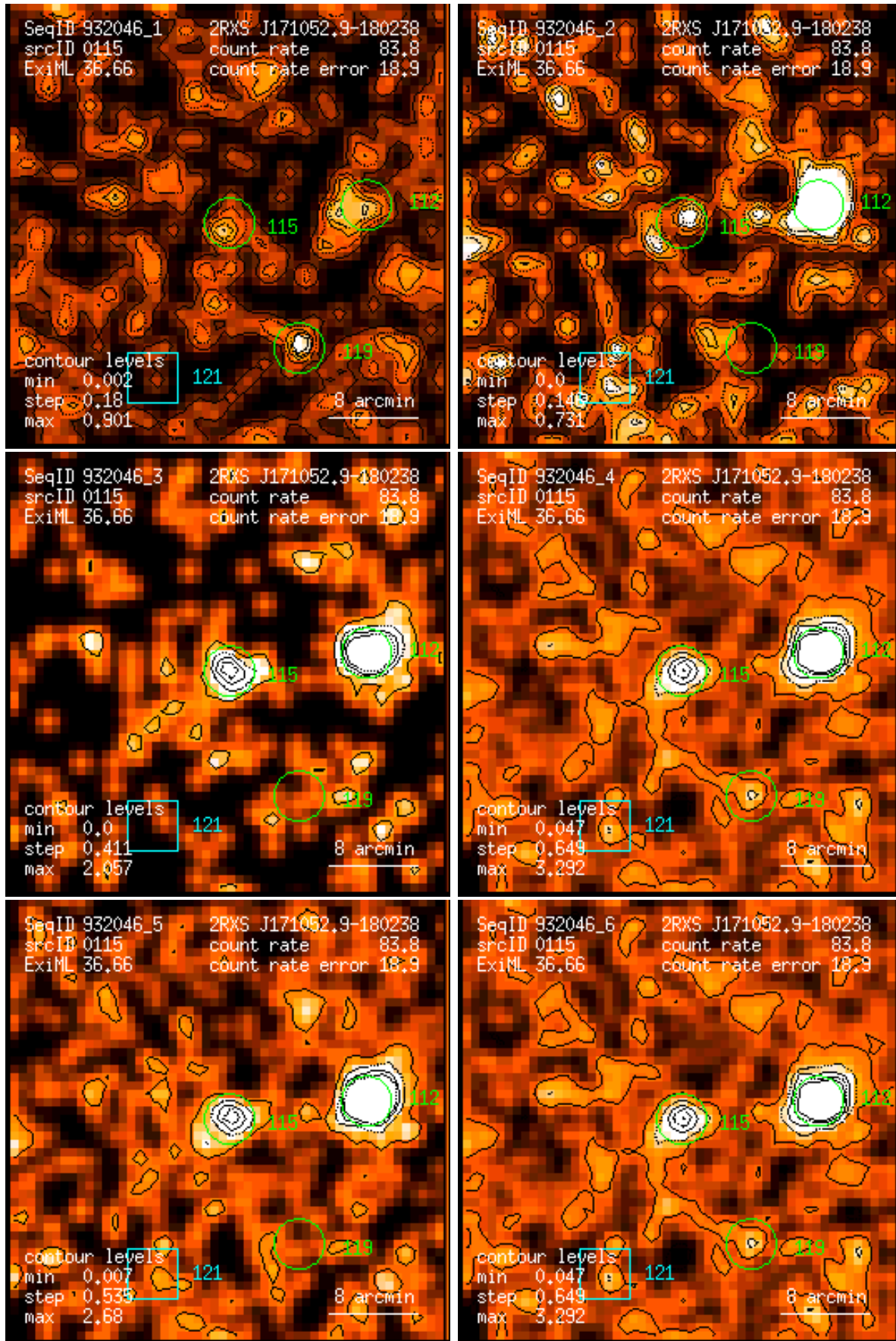
Figure 115: RASS 932046: detection 0115: band rate images, Gaussian filter: (1) PSPC channels 11 – 41, (2) 52 – 90, (3) 91 – 201, (4) 11 – 235, (5) 52 – 201, (6) 11 – 201. Broad band rates in counts/ks. Band rate contour levels in counts/ks/arcmin 2 .
