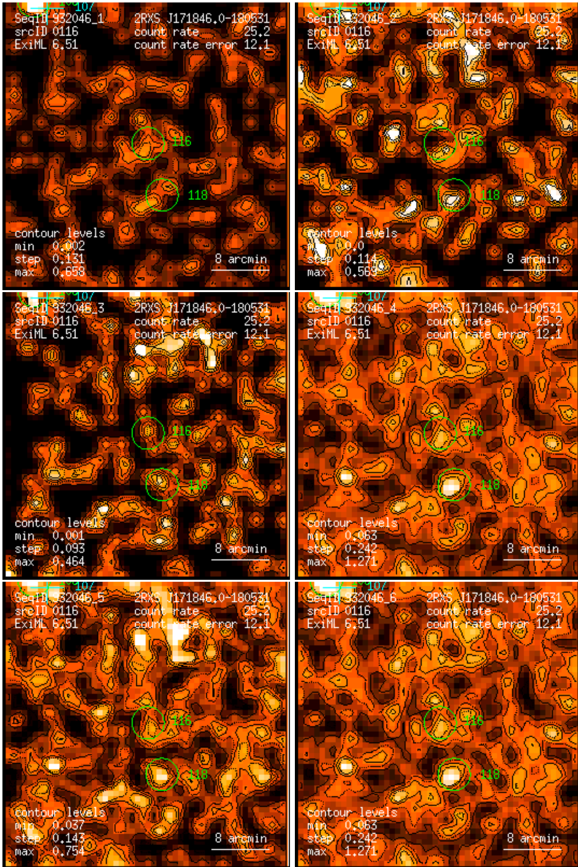
Figure 116: RASS 932046: detection 0116: band rate images, Gaussian filter: (1) PSPC channels 11 – 41, (2) 52 – 90, (3) 91 – 201, (4) 11 – 235, (5) 52 – 201, (6) 11 – 201. Broad band rates in counts/ks. Band rate contour levels in counts/ks/arcmin 2 .
