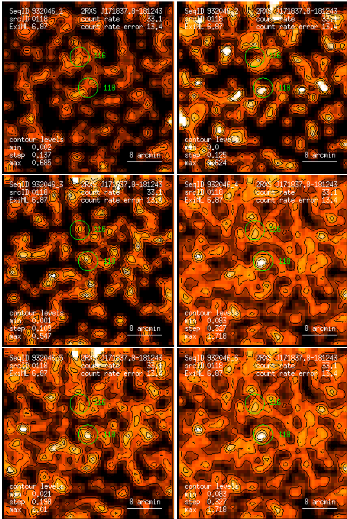
Figure 118: RASS 932046: detection 0118: band rate images, Gaussian filter: (1) PSPC channels 11 – 41, (2) 52 – 90, (3) 91 – 201, (4) 11 – 235, (5) 52 – 201, (6) 11 – 201. Broad band rates in counts/ks. Band rate contour levels in counts/ks/arcmin 2 .
