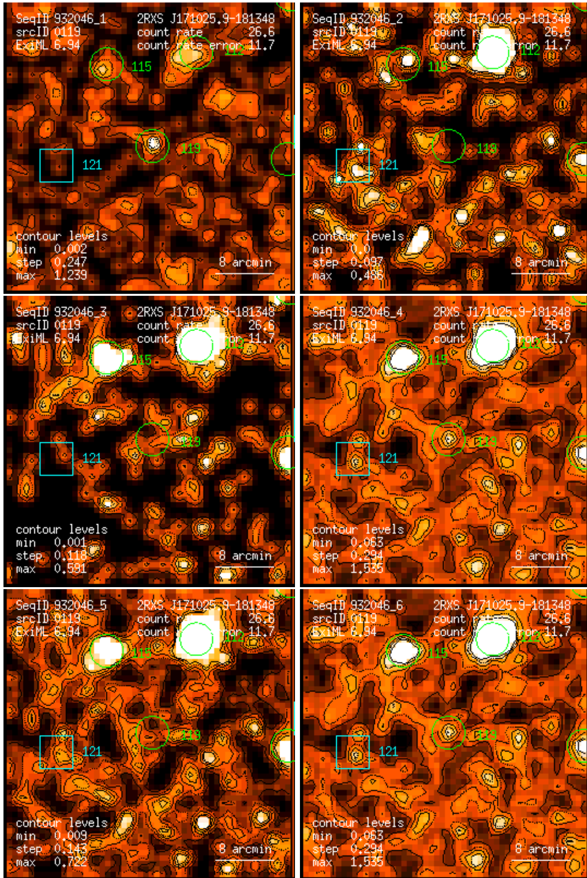
Figure 119: RASS 932046: detection 0119: band rate images, Gaussian filter: (1) PSPC channels 11 – 41, (2) 52 – 90, (3) 91 – 201, (4) 11 – 235, (5) 52 – 201, (6) 11 – 201. Broad band rates in counts/ks. Band rate contour levels in counts/ks/arcmin 2 .
