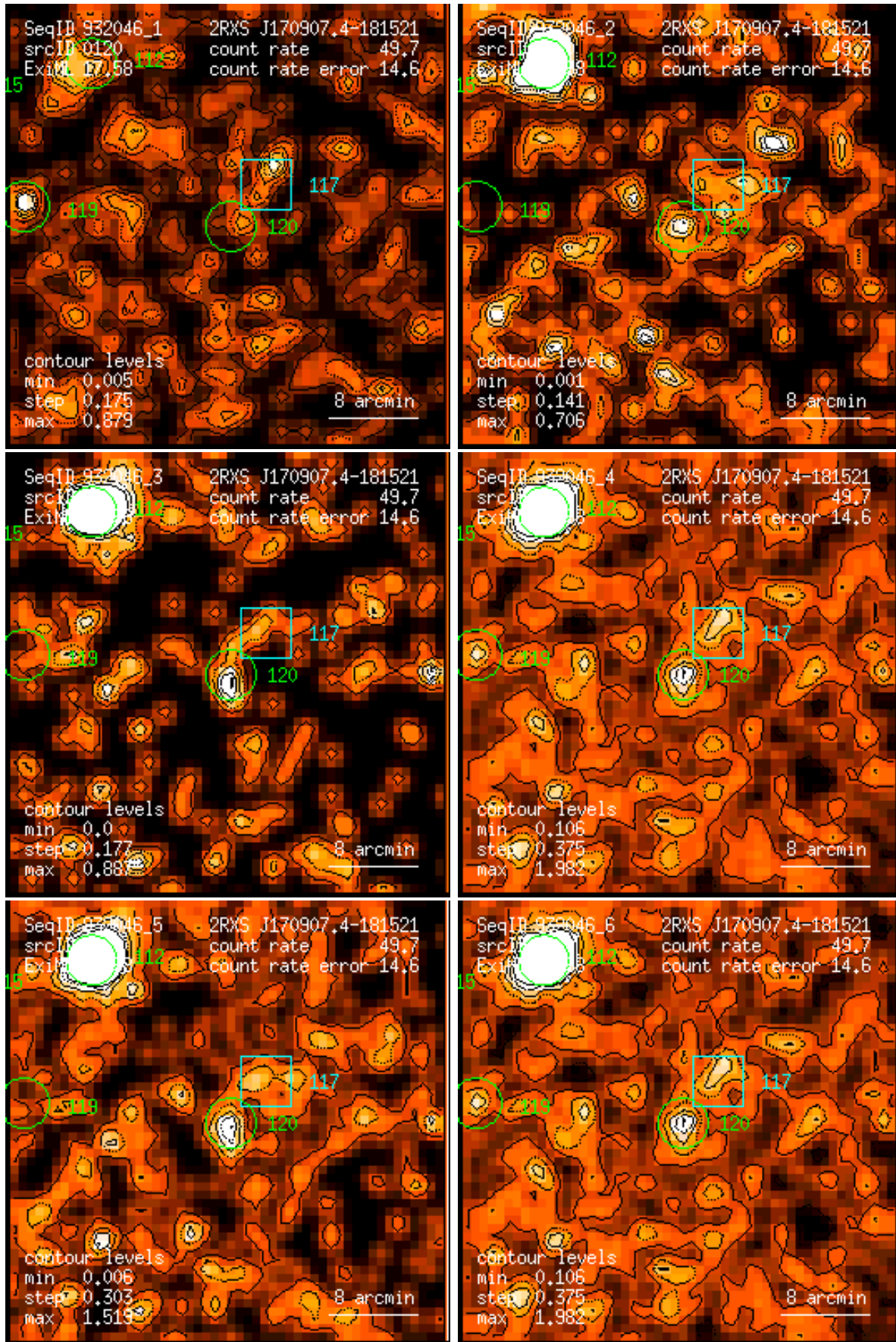
Figure 120: RASS 932046: detection 0120: band rate images, Gaussian filter: (1) PSPC channels 11 – 41, (2) 52 – 90, (3) 91 – 201, (4) 11 – 235, (5) 52 – 201, (6) 11 – 201. Broad band rates in counts/ks. Band rate contour levels in counts/ks/arcmin 2 .
