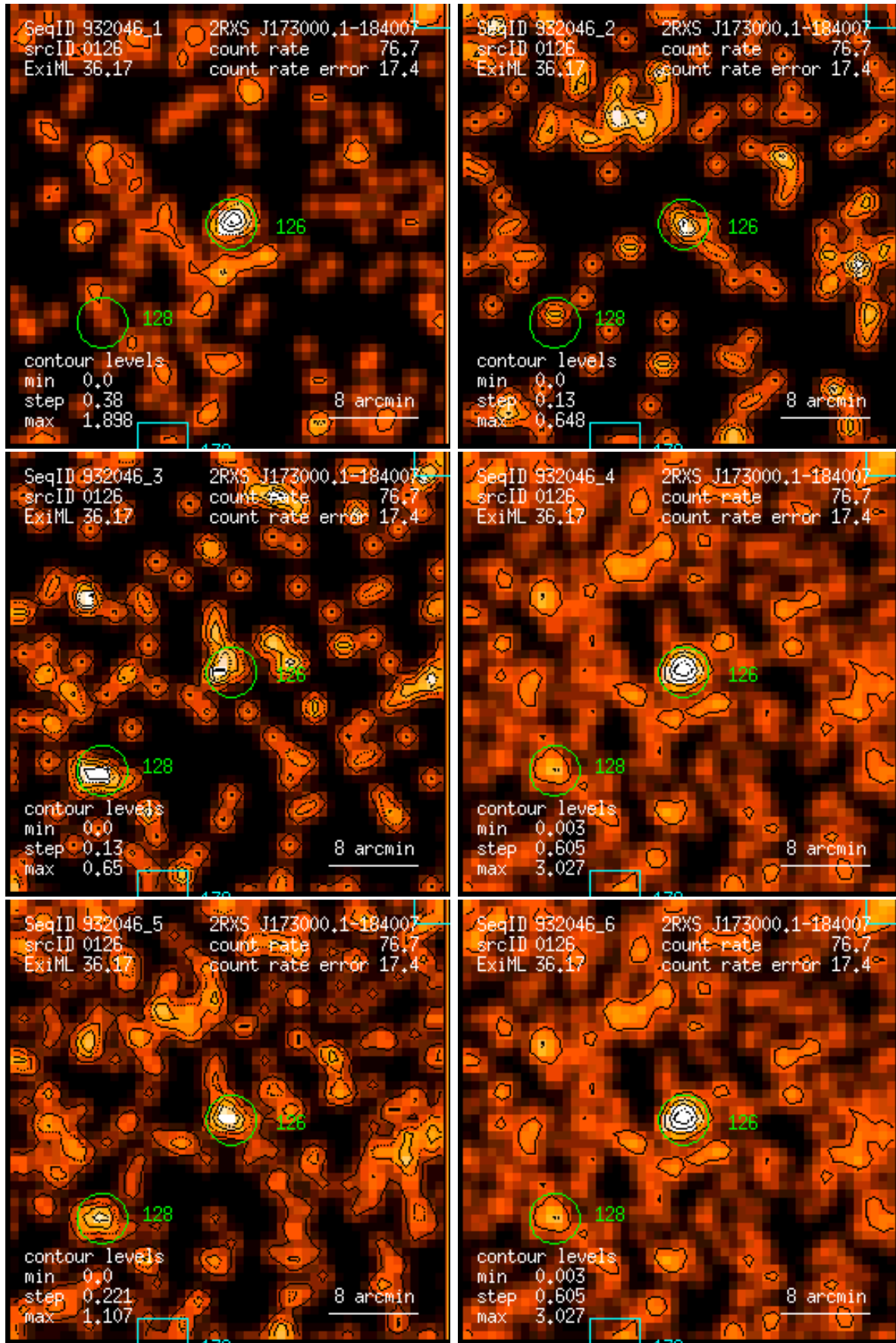
Figure 126: RASS 932046: detection 0126: band rate images, Gaussian filter: (1) PSPC channels 11 – 41, (2) 52 – 90, (3) 91 – 201, (4) 11 – 235, (5) 52 – 201, (6) 11 – 201. Broad band rates in counts/ks. Band rate contour levels in counts/ks/arcmin 2 .
