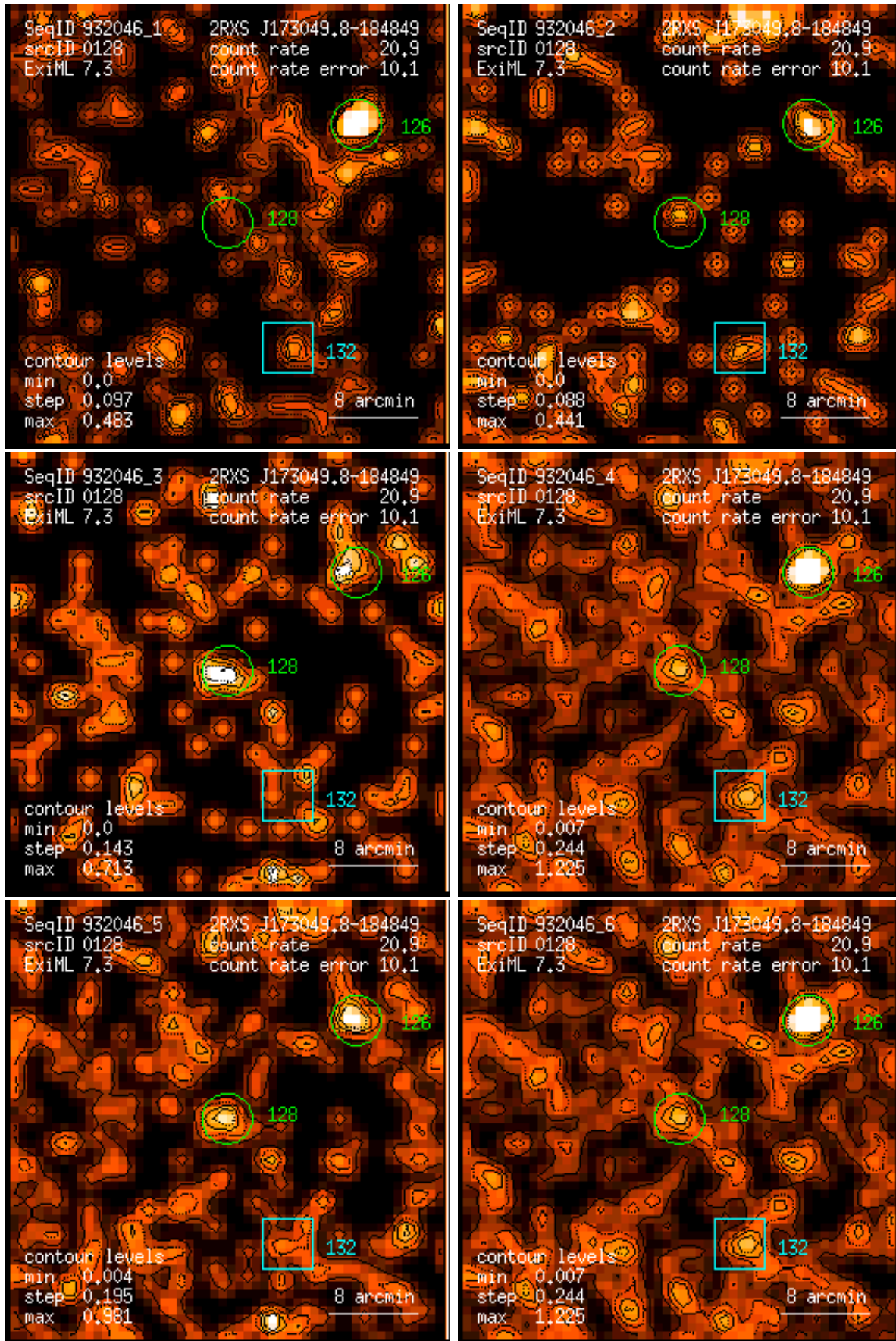
Figure 128: RASS 932046: detection 0128: band rate images, Gaussian filter: (1) PSPC channels 11 – 41, (2) 52 – 90, (3) 91 – 201, (4) 11 – 235, (5) 52 – 201, (6) 11 – 201. Broad band rates in counts/ks. Band rate contour levels in counts/ks/arcmin 2 .
