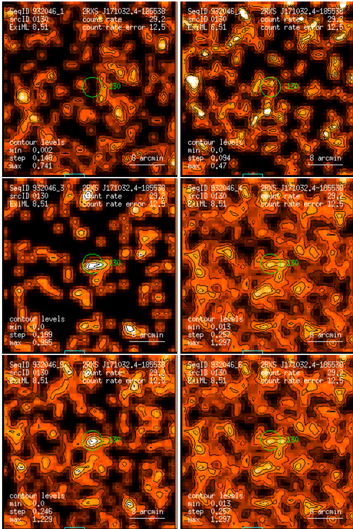
Figure 130: RASS 932046: detection 0130: band rate images, Gaussian filter: (1) PSPC channels 11 – 41, (2) 52 – 90, (3) 91 – 201, (4) 11 – 235, (5) 52 – 201, (6) 11 – 201. Broad band rates in counts/ks. Band rate contour levels in counts/ks/arcmin 2 .
