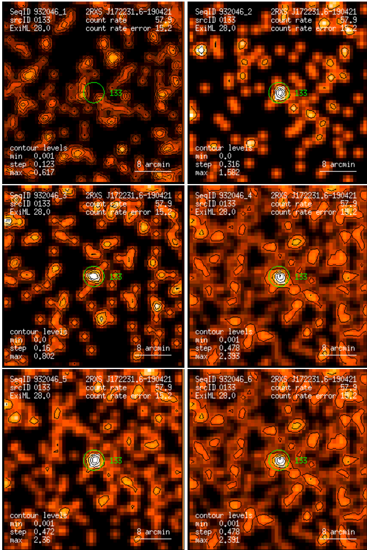
Figure 133: RASS 932046: detection 0133: band rate images, Gaussian filter: (1) PSPC channels 11 – 41, (2) 52 – 90, (3) 91 – 201, (4) 11 – 235, (5) 52 – 201, (6) 11 – 201. Broad band rates in counts/ks. Band rate contour levels in counts/ks/arcmin 2 .
