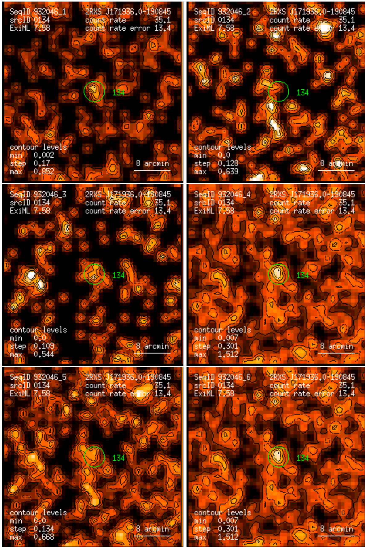
Figure 134: RASS 932046: detection 0134: band rate images, Gaussian filter: (1) PSPC channels 11 – 41, (2) 52 – 90, (3) 91 – 201, (4) 11 – 235, (5) 52 – 201, (6) 11 – 201. Broad band rates in counts/ks. Band rate contour levels in counts/ks/arcmin 2 .
