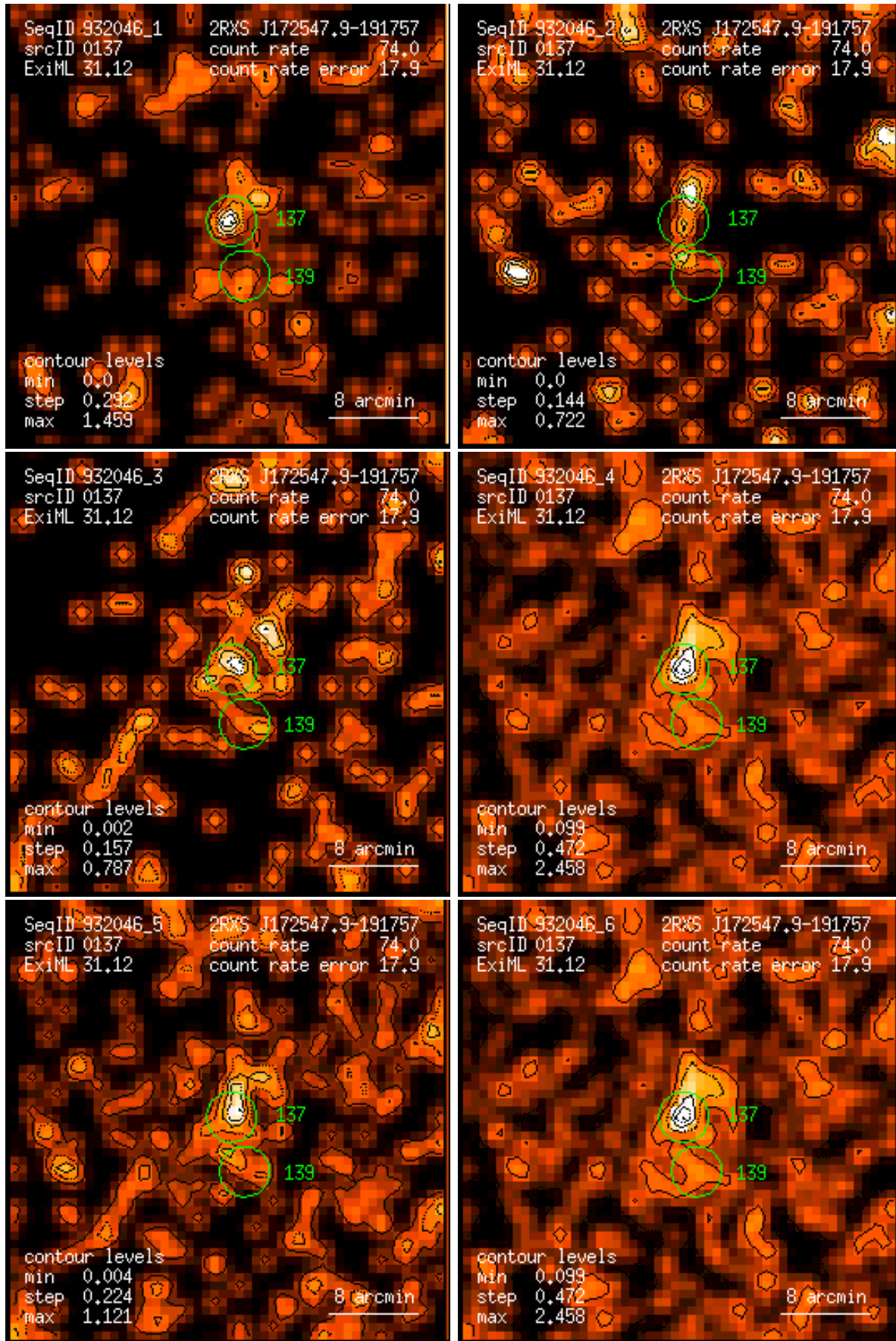
Figure 137: RASS 932046: detection 0137: band rate images, Gaussian filter: (1) PSPC channels 11 – 41, (2) 52 – 90, (3) 91 – 201, (4) 11 – 235, (5) 52 – 201, (6) 11 – 201. Broad band rates in counts/ks. Band rate contour levels in counts/ks/arcmin 2 .
