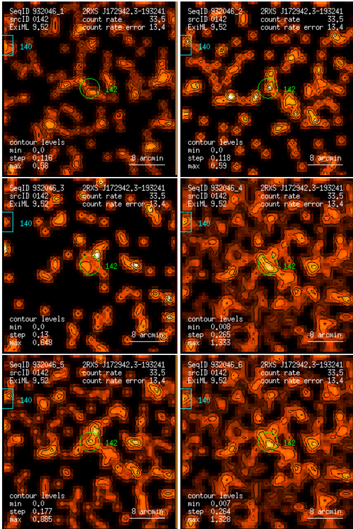
Figure 142: RASS 932046: detection 0142: band rate images, Gaussian filter: (1) PSPC channels 11 – 41, (2) 52 – 90, (3) 91 – 201, (4) 11 – 235, (5) 52 – 201, (6) 11 – 201. Broad band rates in counts/ks. Band rate contour levels in counts/ks/arcmin 2 .
