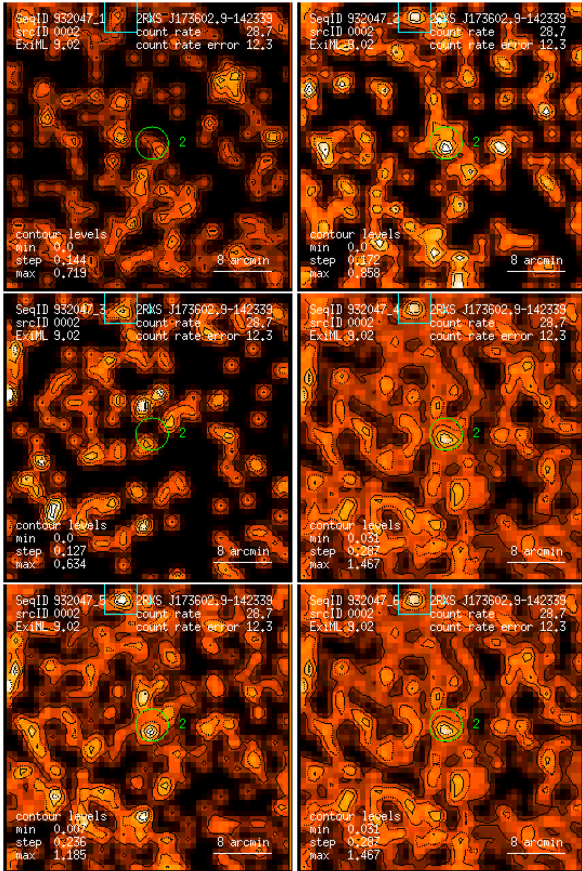
Figure 2: RASS 932047: detection 0002: band rate images, Gaussian filter: (1) PSPC channels 11 – 41, (2) 52 – 90, (3) 91 – 201, (4) 11 – 235, (5) 52 – 201, (6) 11 – 201. Broad band rates in counts/ks. Band rate contour levels in counts/ks/arcmin 2 .
