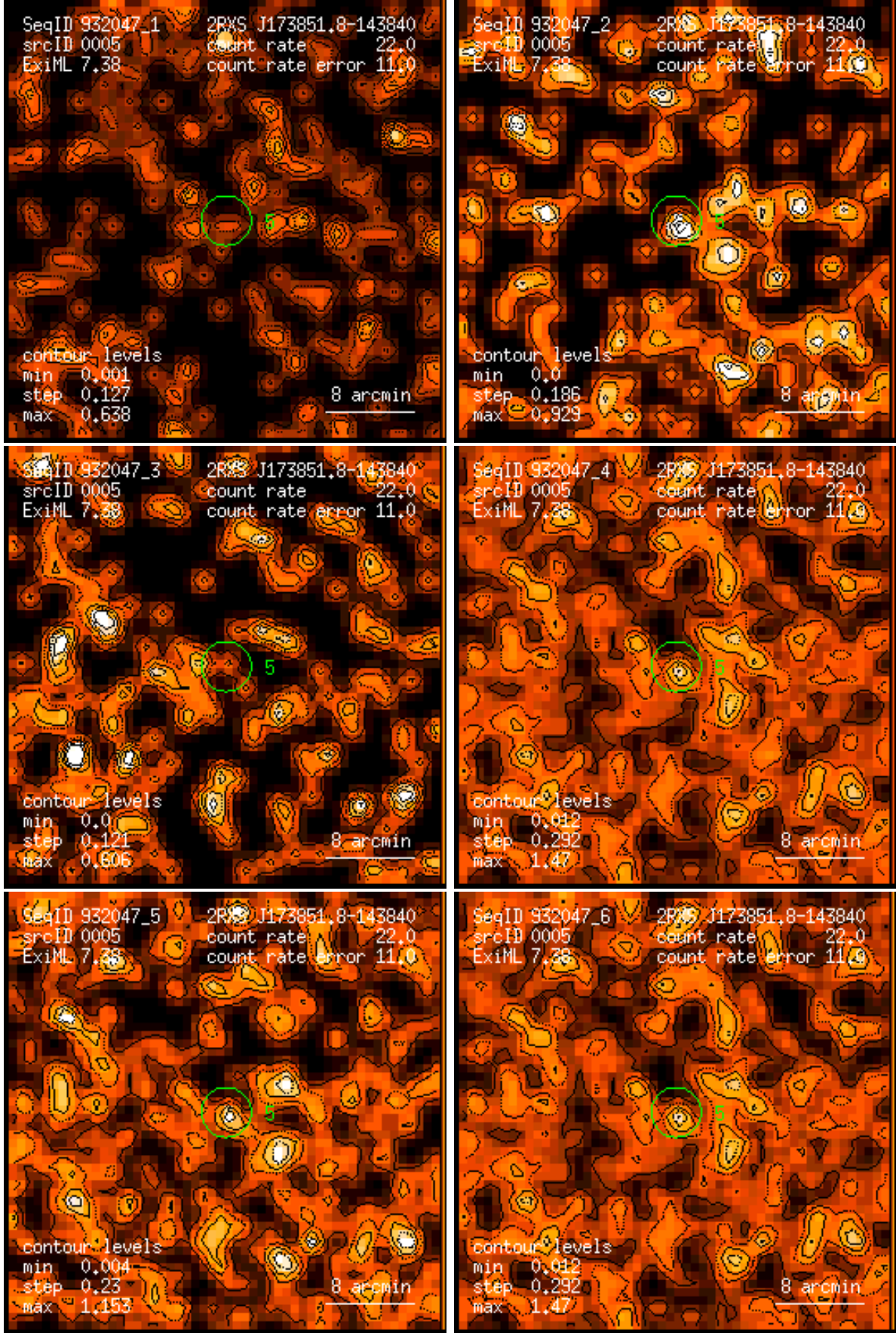
Figure 5: RASS 932047: detection 0005: band rate images, Gaussian filter: (1) PSPC channels 11 – 41, (2) 52 – 90, (3) 91 – 201, (4) 11 – 235, (5) 52 – 201, (6) 11 – 201. Broad band rates in counts/ks. Band rate contour levels in counts/ks/arcmin 2 .
