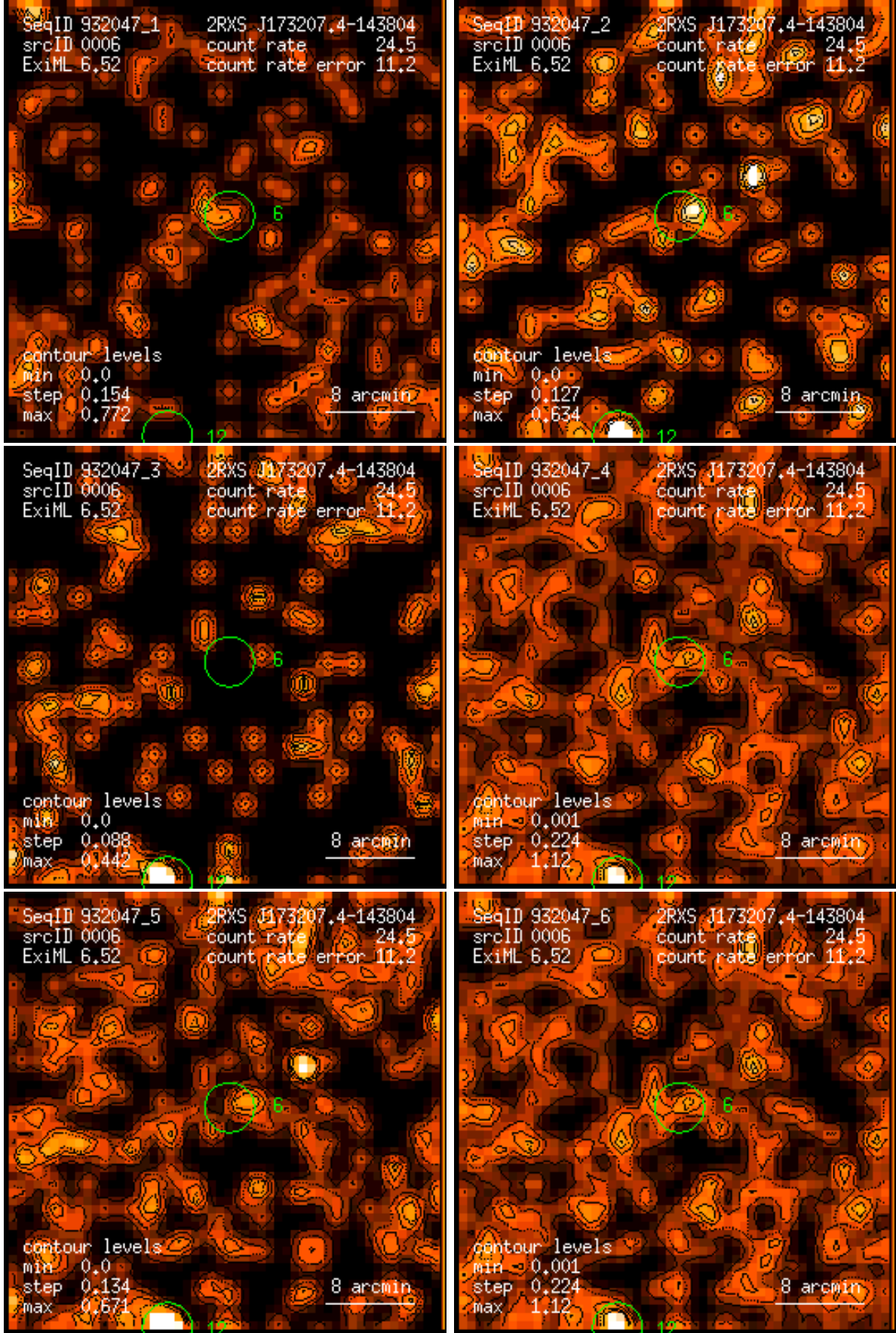
Figure 6: RASS 932047: detection 0006: band rate images, Gaussian filter: (1) PSPC channels 11 – 41, (2) 52 – 90, (3) 91 – 201, (4) 11 – 235, (5) 52 – 201, (6) 11 – 201. Broad band rates in counts/ks. Band rate contour levels in counts/ks/arcmin 2 .
