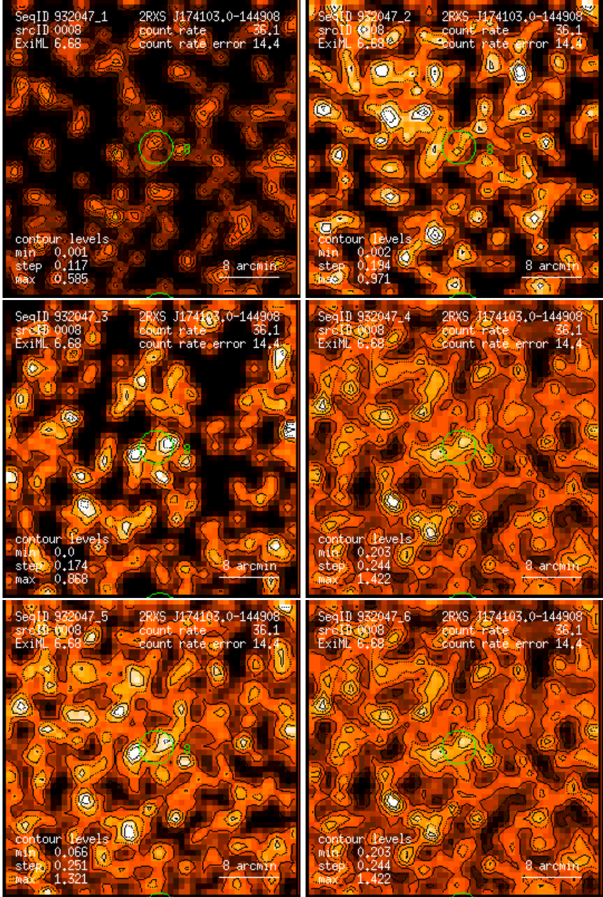
Figure 8: RASS 932047: detection 0008: band rate images, Gaussian filter: (1) PSPC channels 11 – 41, (2) 52 – 90, (3) 91 – 201, (4) 11 – 235, (5) 52 – 201, (6) 11 – 201. Broad band rates in counts/ks. Band rate contour levels in counts/ks/arcmin 2 .
