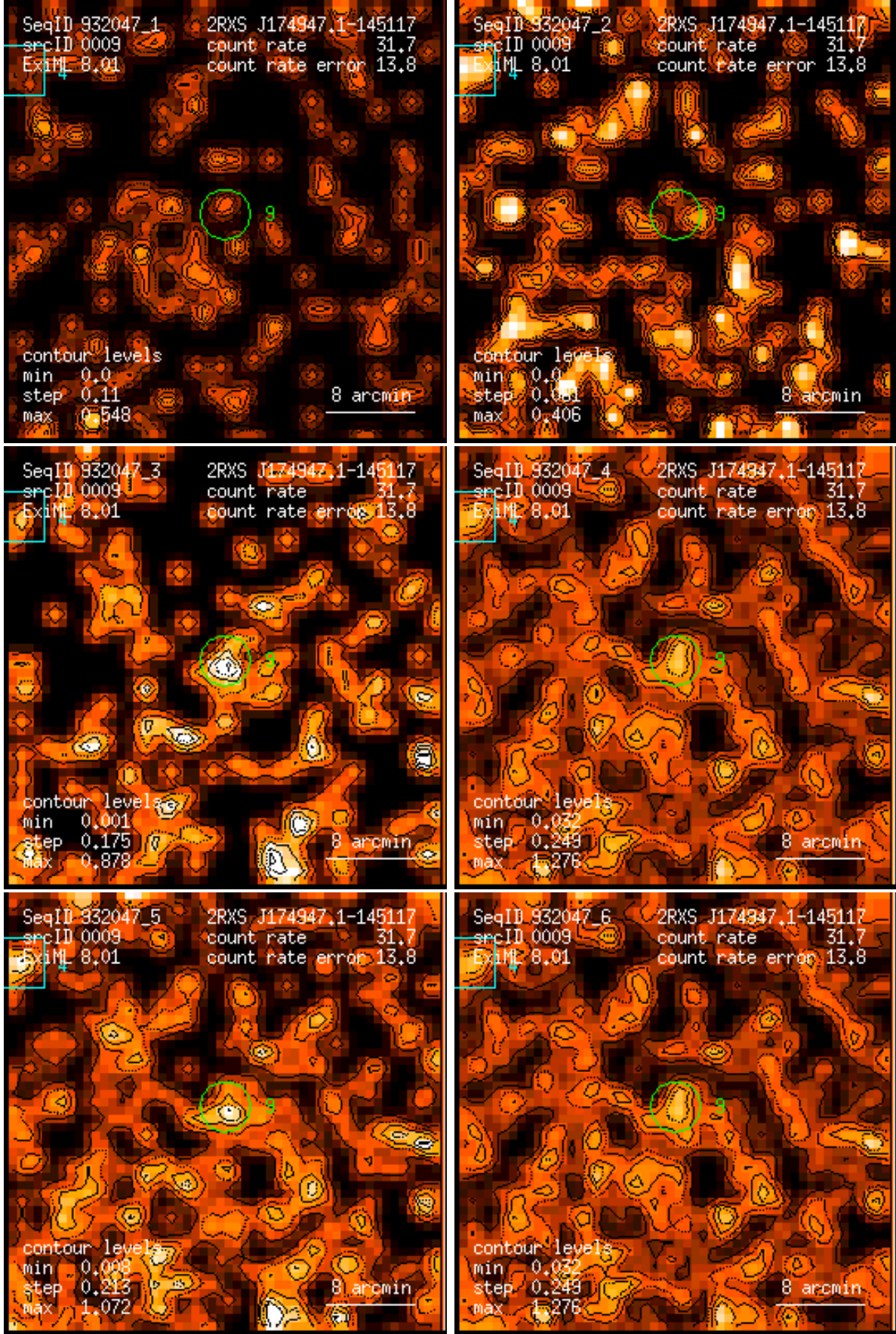
Figure 9: RASS 932047: detection 0009: band rate images, Gaussian filter: (1) PSPC channels 11 – 41, (2) 52 – 90, (3) 91 – 201, (4) 11 – 235, (5) 52 – 201, (6) 11 – 201. Broad band rates in counts/ks. Band rate contour levels in counts/ks/arcmin 2 .
