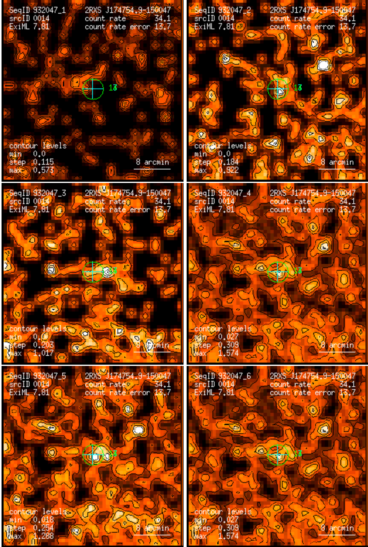
Figure 14: RASS 932047: detection 0014: band rate images, Gaussian filter: (1) PSPC channels 11 – 41, (2) 52 – 90, (3) 91 – 201, (4) 11 – 235, (5) 52 – 201, (6) 11 – 201. Broad band rates in counts/ks. Band rate contour levels in counts/ks/arcmin 2 .
