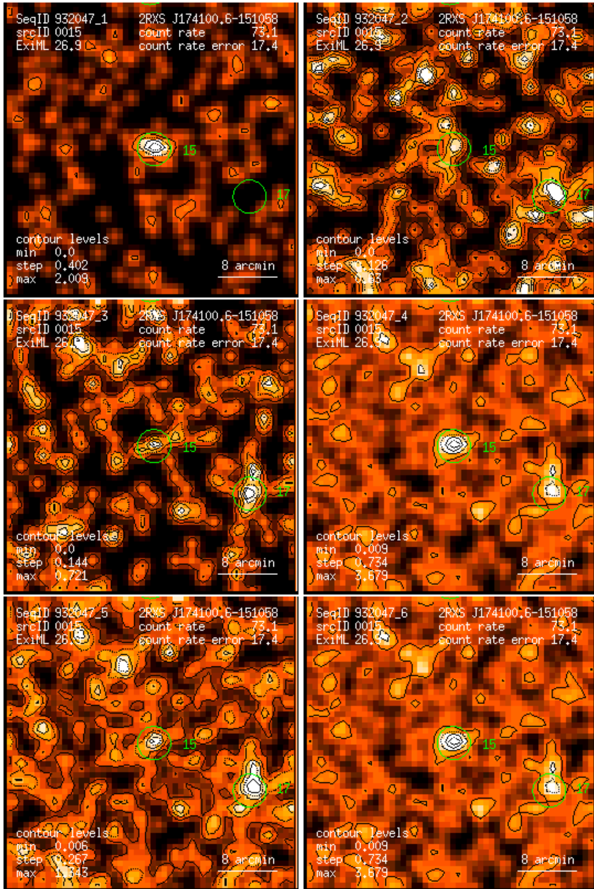
Figure 15: RASS 932047: detection 0015: band rate images, Gaussian filter: (1) PSPC channels 11 – 41, (2) 52 – 90, (3) 91 – 201, (4) 11 – 235, (5) 52 – 201, (6) 11 – 201. Broad band rates in counts/ks. Band rate contour levels in counts/ks/arcmin 2 .
