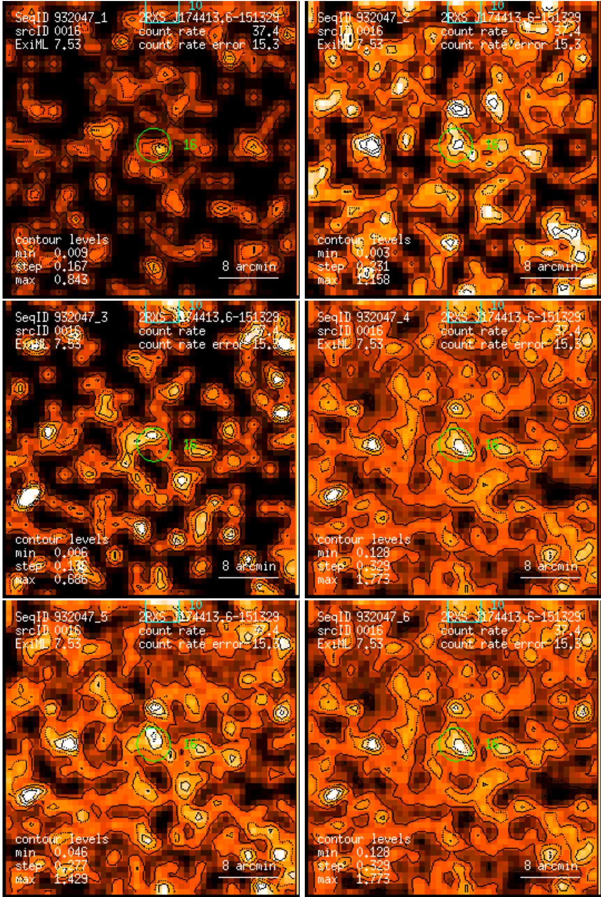
Figure 16: RASS 932047: detection 0016: band rate images, Gaussian filter: (1) PSPC channels 11 – 41, (2) 52 – 90, (3) 91 – 201, (4) 11 – 235, (5) 52 – 201, (6) 11 – 201. Broad band rates in counts/ks. Band rate contour levels in counts/ks/arcmin 2 .
