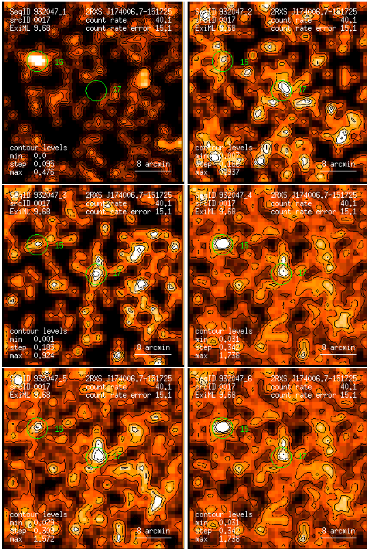
Figure 17: RASS 932047: detection 0017: band rate images, Gaussian filter: (1) PSPC channels 11 – 41, (2) 52 – 90, (3) 91 – 201, (4) 11 – 235, (5) 52 – 201, (6) 11 – 201. Broad band rates in counts/ks. Band rate contour levels in counts/ks/arcmin 2 .
