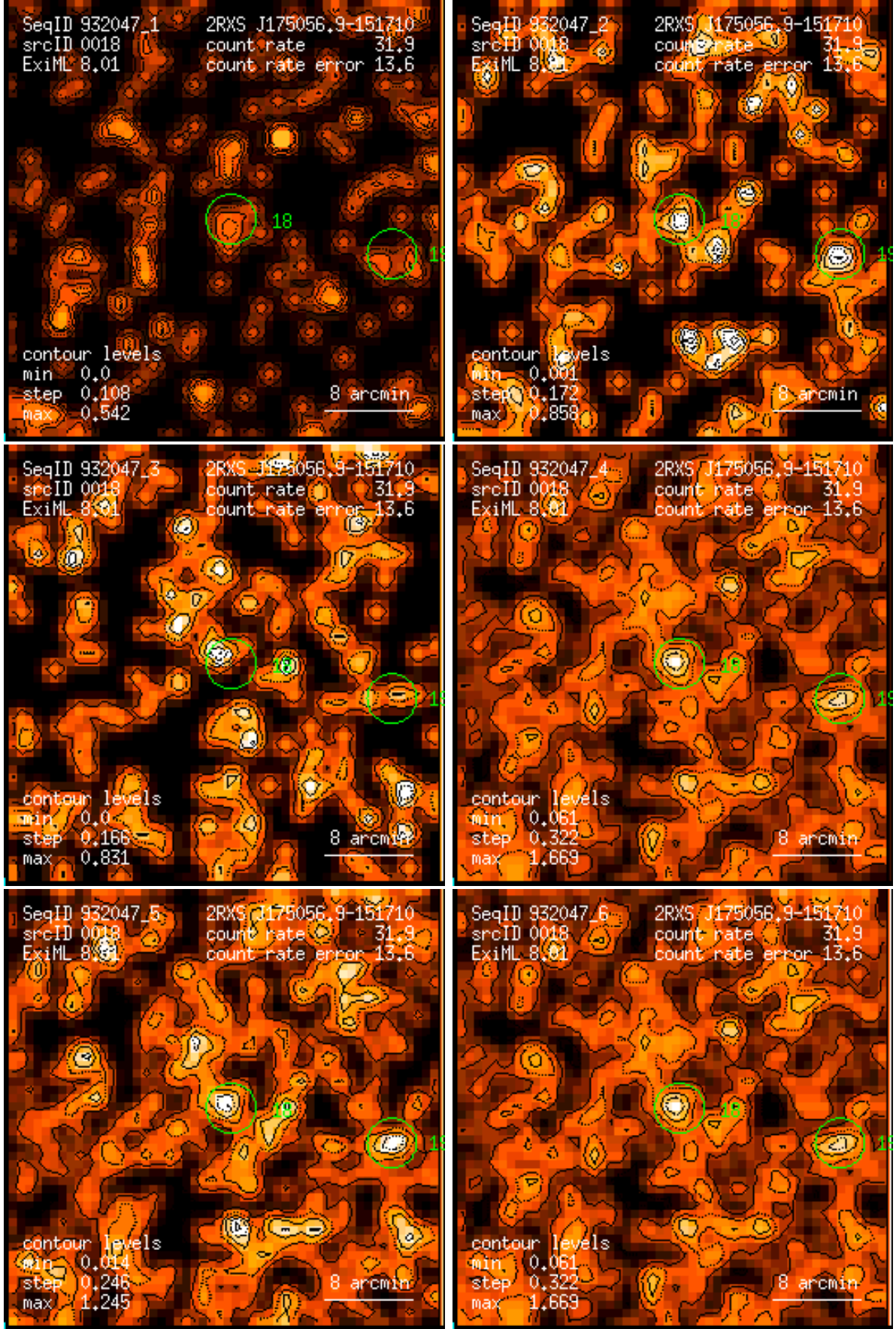
Figure 18: RASS 932047: detection 0018: band rate images, Gaussian filter: (1) PSPC channels 11 – 41, (2) 52 – 90, (3) 91 – 201, (4) 11 – 235, (5) 52 – 201, (6) 11 – 201. Broad band rates in counts/ks. Band rate contour levels in counts/ks/arcmin 2 .
