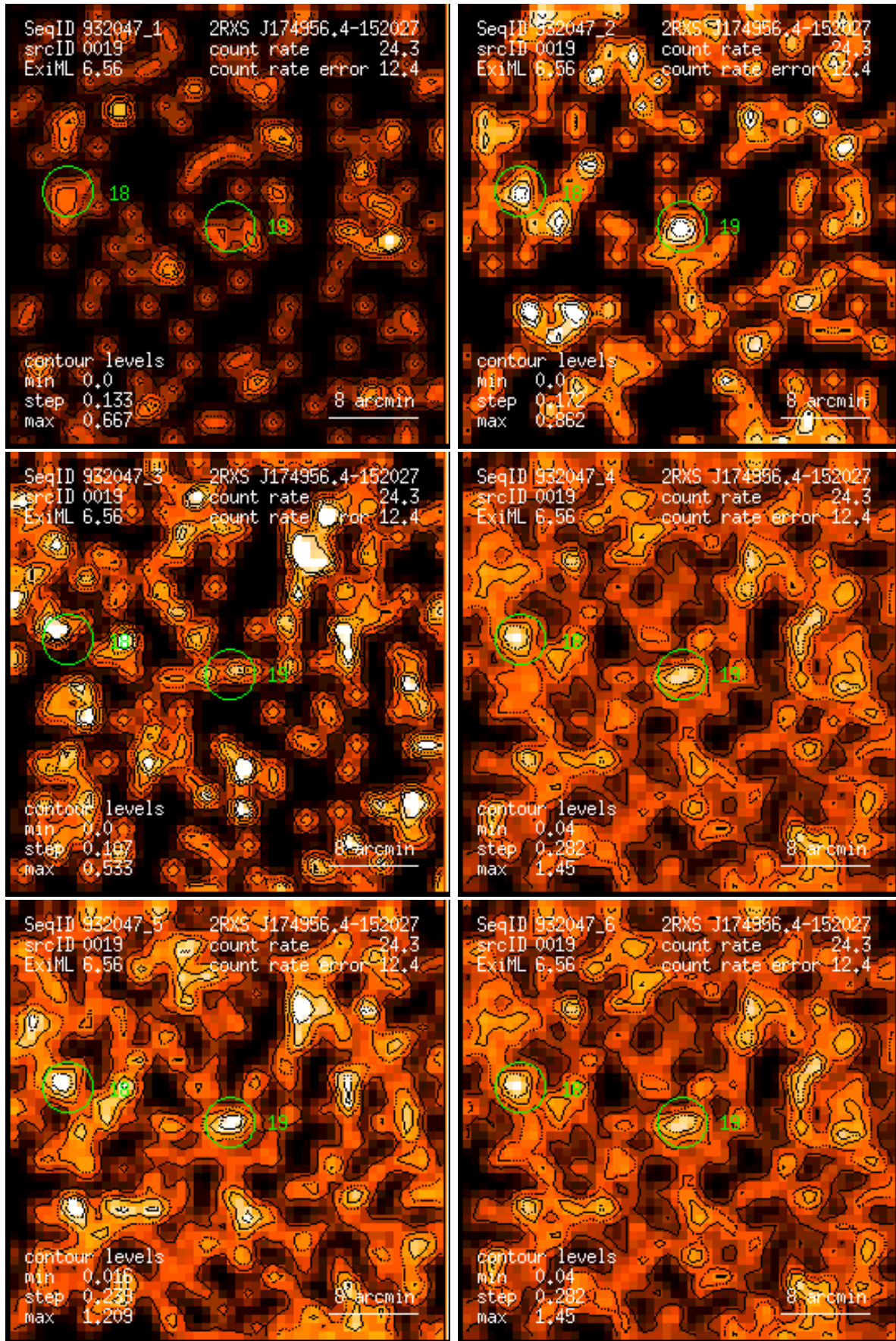
Figure 19: RASS 932047: detection 0019: band rate images, Gaussian filter: (1) PSPC channels 11 – 41, (2) 52 – 90, (3) 91 – 201, (4) 11 – 235, (5) 52 – 201, (6) 11 – 201. Broad band rates in counts/ks. Band rate contour levels in counts/ks/arcmin 2 .
