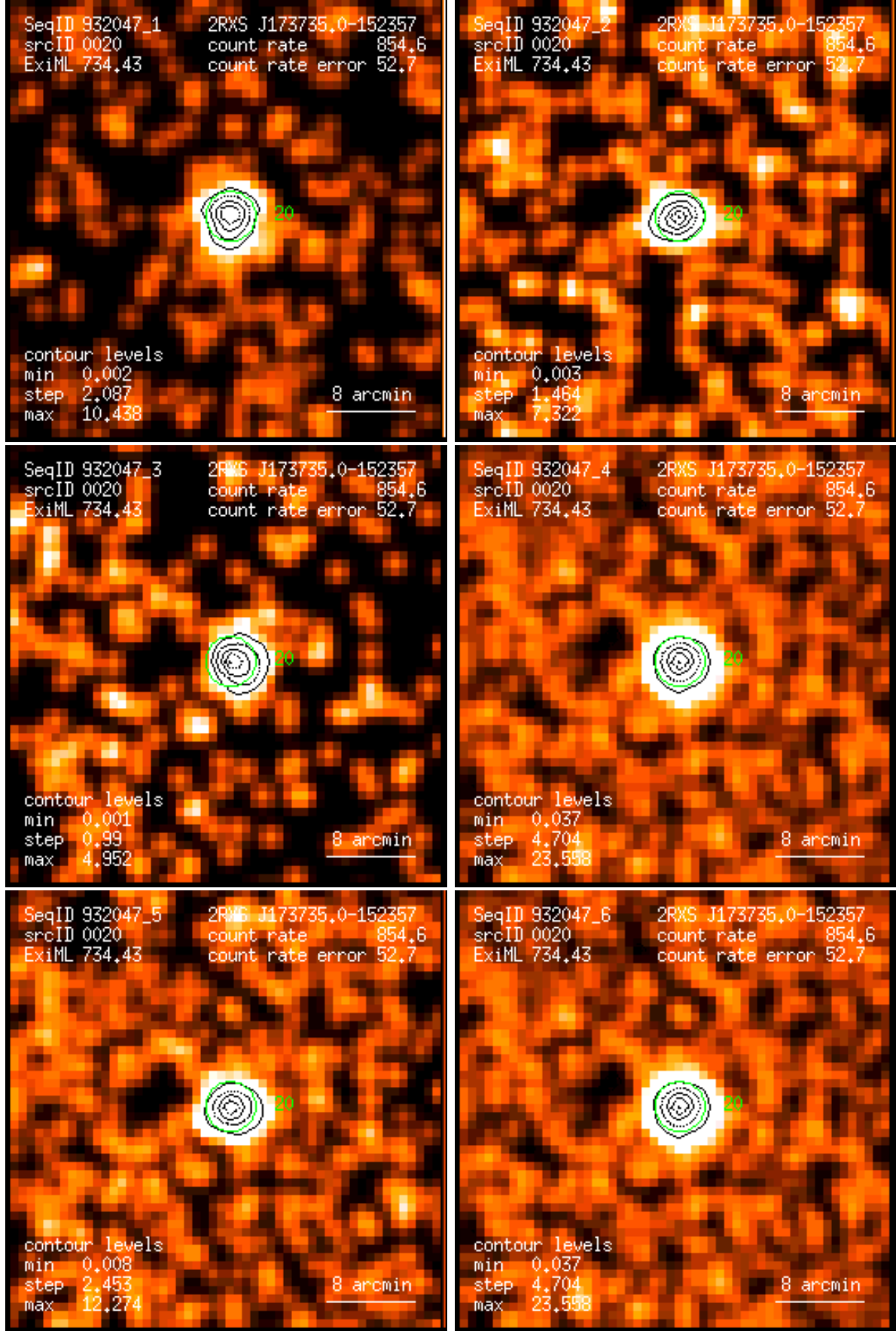
Figure 20: RASS 932047: detection 0020: band rate images, Gaussian filter: (1) PSPC channels 11 – 41, (2) 52 – 90, (3) 91 – 201, (4) 11 – 235, (5) 52 – 201, (6) 11 – 201. Broad band rates in counts/ks. Band rate contour levels in counts/ks/arcmin 2 .
