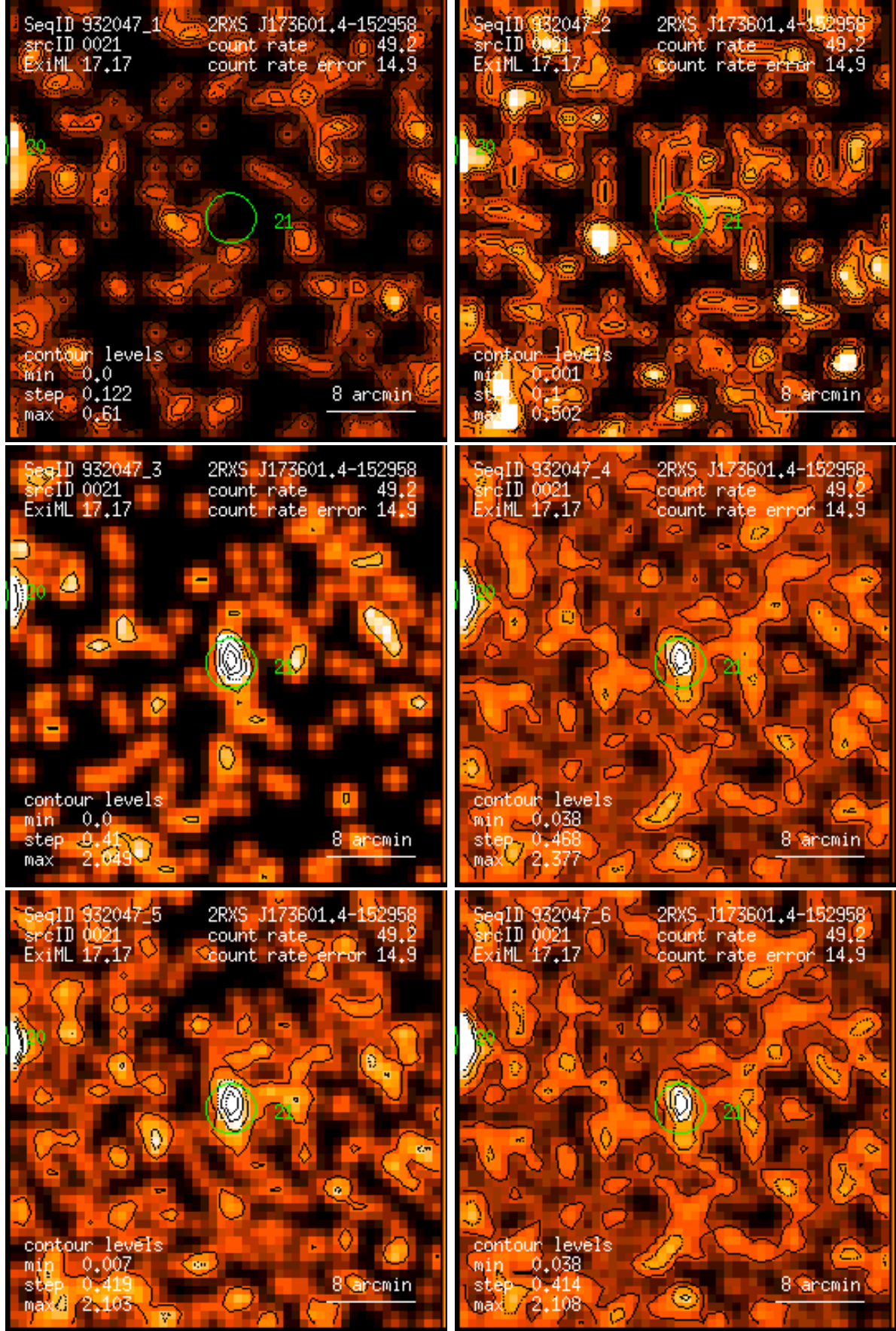
Figure 21: RASS 932047: detection 0021: band rate images, Gaussian filter: (1) PSPC channels 11 – 41, (2) 52 – 90, (3) 91 – 201, (4) 11 – 235, (5) 52 – 201, (6) 11 – 201. Broad band rates in counts/ks. Band rate contour levels in counts/ks/arcmin 2 .
