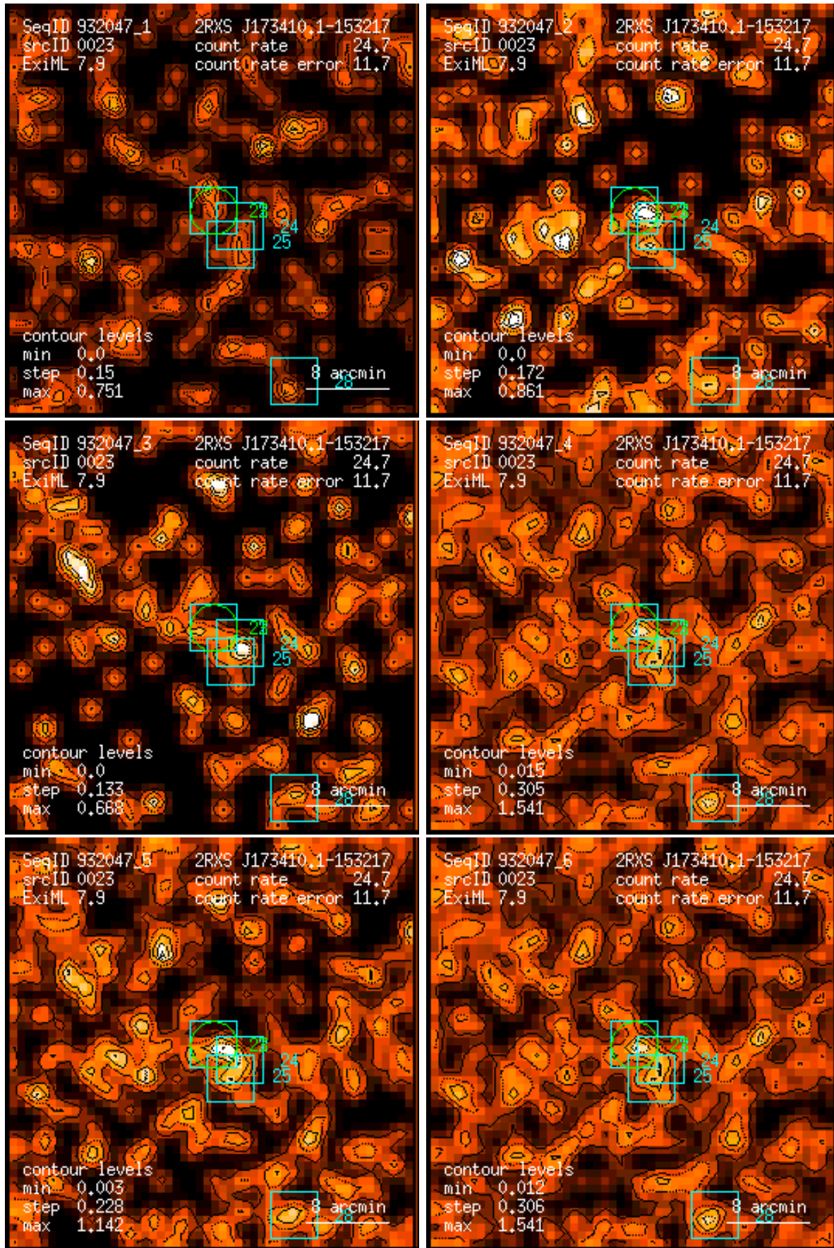
Figure 23: RASS 932047: detection 0023: band rate images, Gaussian filter: (1) PSPC channels 11 – 41, (2) 52 – 90, (3) 91 – 201, (4) 11 – 235, (5) 52 – 201, (6) 11 – 201. Broad band rates in counts/ks. Band rate contour levels in counts/ks/arcmin 2 .
